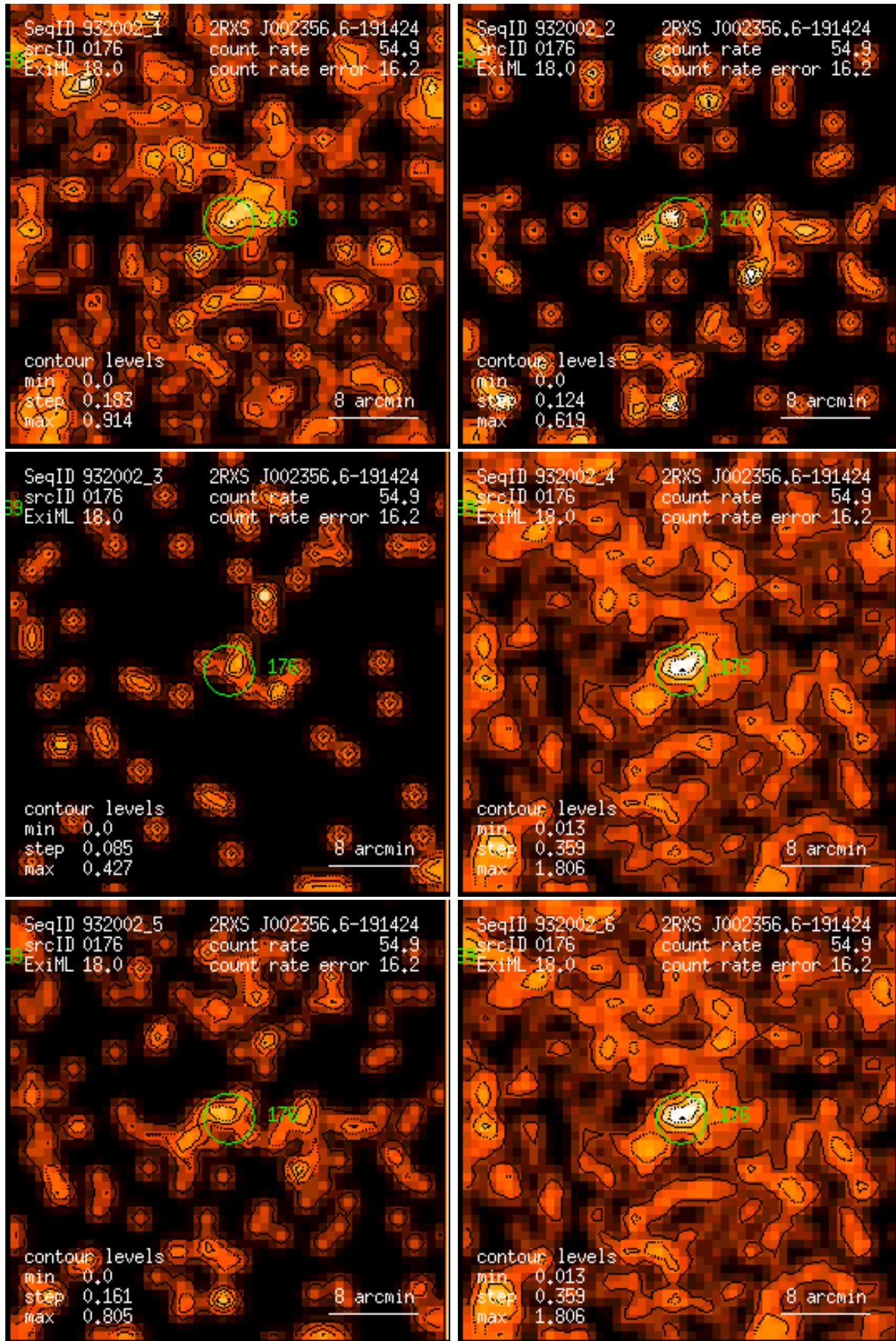
Figure 176: RASS 932002: detection 0176: band rate images, Gaussian filter: (1) PSPC channels 11 – 41, (2) 52 – 90, (3) 91 – 201, (4) 11 – 235, (5) 52 – 201, (6) 11 – 201. Broad band rates in counts/ks. Band rate contour levels in counts/ks/arcmin 2 .
