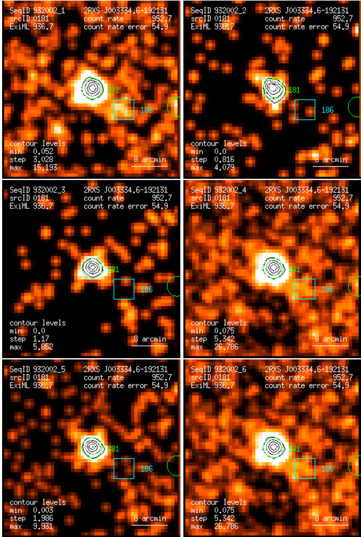
Figure 181: RASS 932002: detection 0181: band rate images, Gaussian filter: (1) PSPC channels 11 – 41, (2) 52 – 90, (3) 91 – 201, (4) 11 – 235, (5) 52 – 201, (6) 11 – 201. Broad band rates in counts/ks. Band rate contour levels in counts/ks/arcmin 2 .
