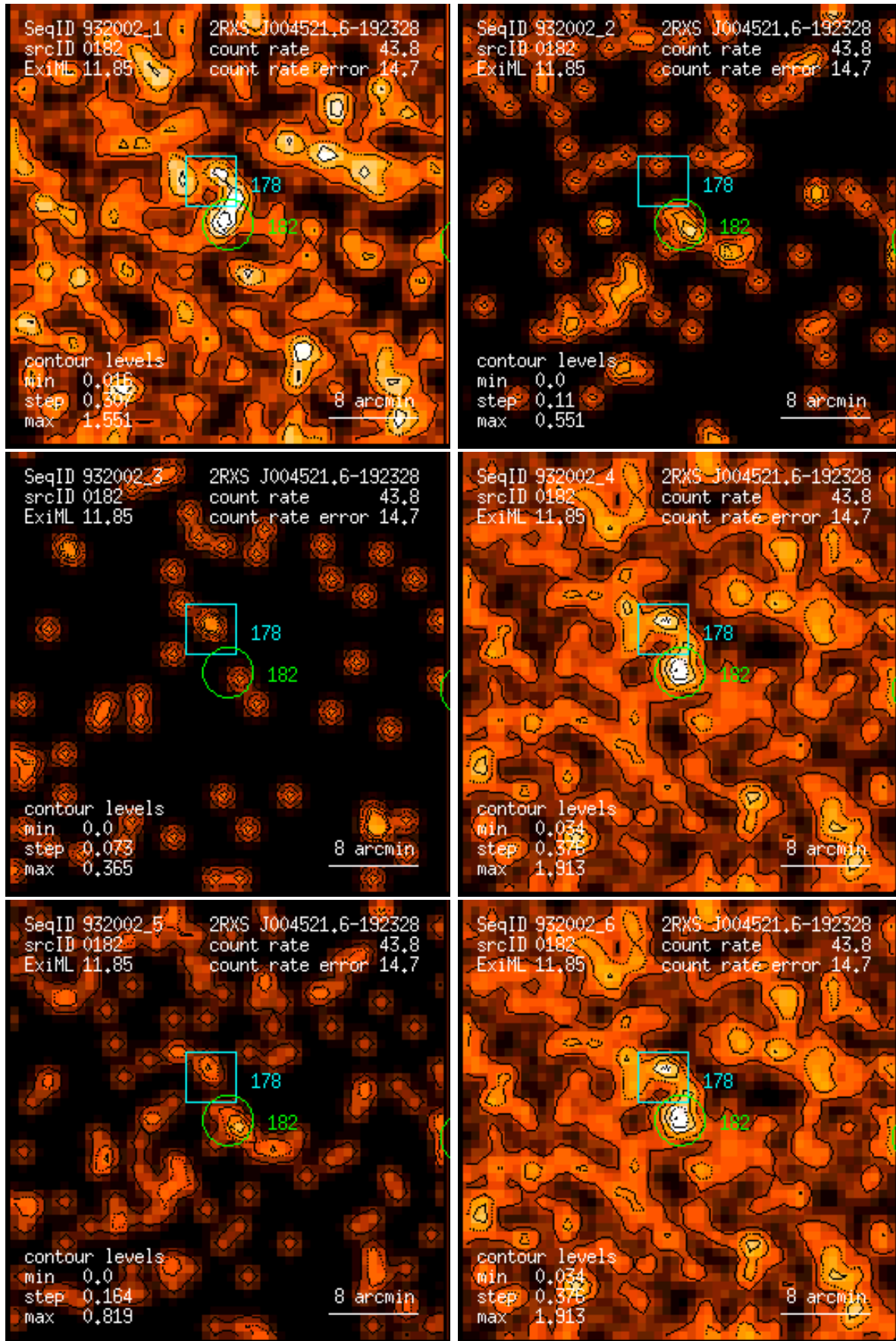
Figure 182: RASS 932002: detection 0182: band rate images, Gaussian filter: (1) PSPC channels 11 – 41, (2) 52 – 90, (3) 91 – 201, (4) 11 – 235, (5) 52 – 201, (6) 11 – 201. Broad band rates in counts/ks. Band rate contour levels in counts/ks/arcmin 2 .
