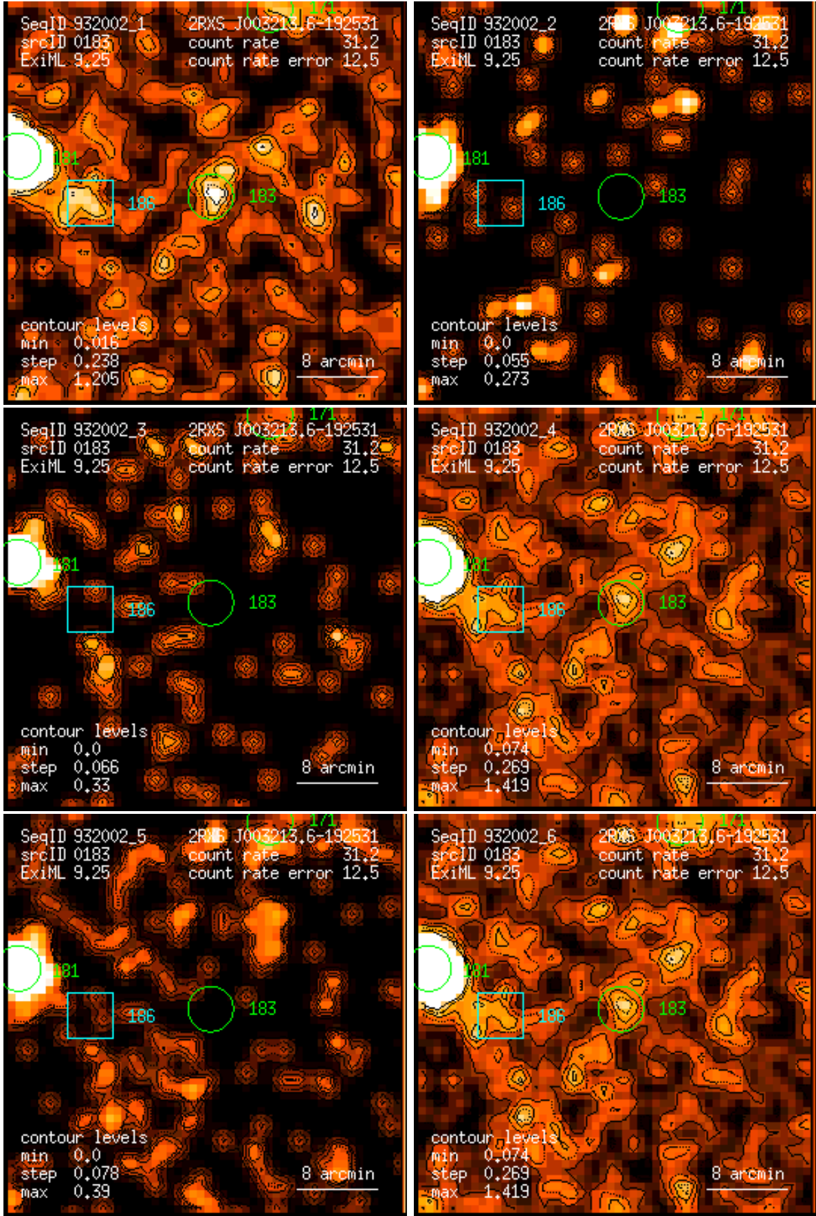
Figure 183: RASS 932002: detection 0183: band rate images, Gaussian filter: (1) PSPC channels 11 – 41, (2) 52 – 90, (3) 91 – 201, (4) 11 – 235, (5) 52 – 201, (6) 11 – 201. Broad band rates in counts/ks. Band rate contour levels in counts/ks/arcmin 2 .
