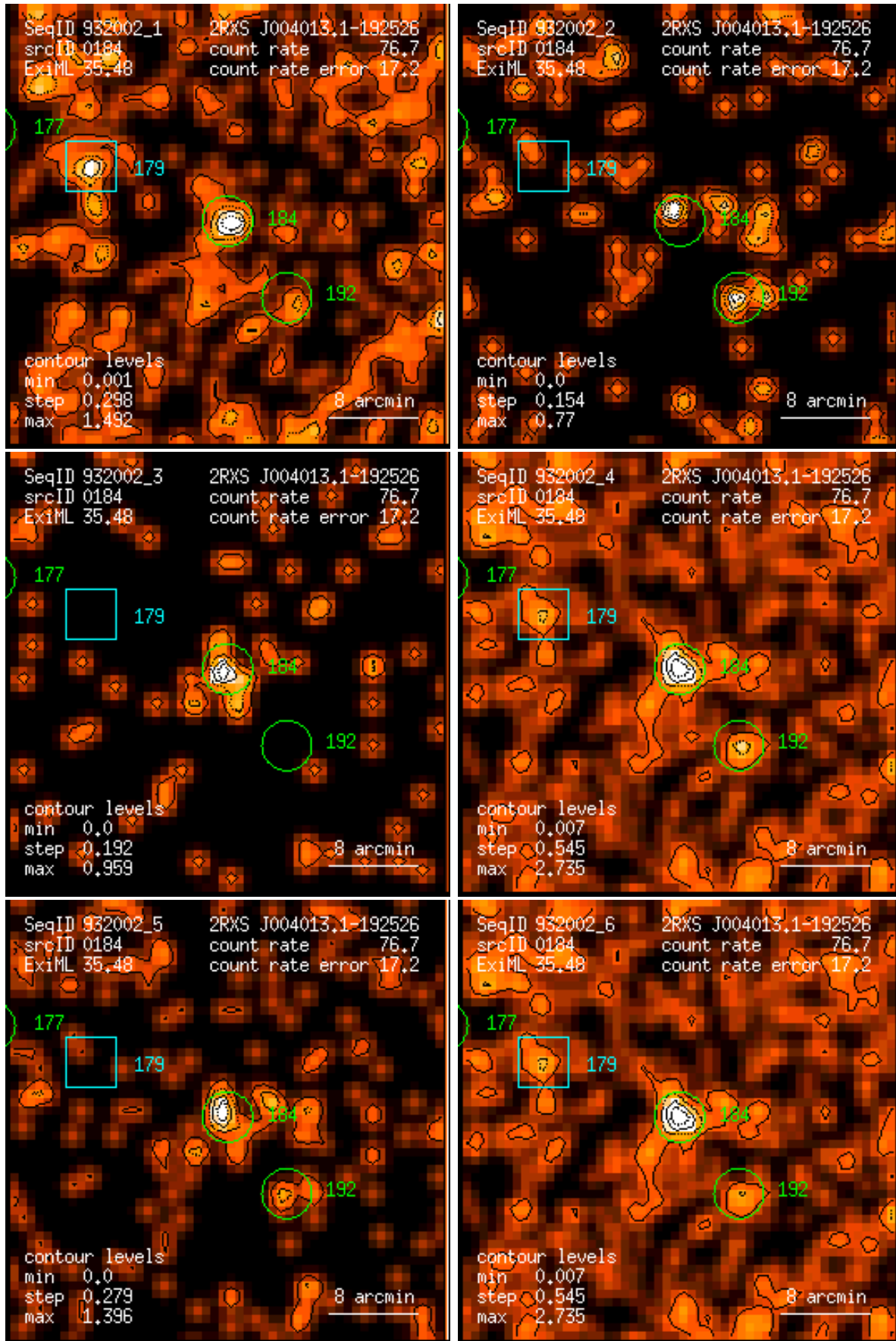
Figure 184: RASS 932002: detection 0184: band rate images, Gaussian filter: (1) PSPC channels 11 – 41, (2) 52 – 90, (3) 91 – 201, (4) 11 – 235, (5) 52 – 201, (6) 11 – 201. Broad band rates in counts/ks. Band rate contour levels in counts/ks/arcmin 2 .
