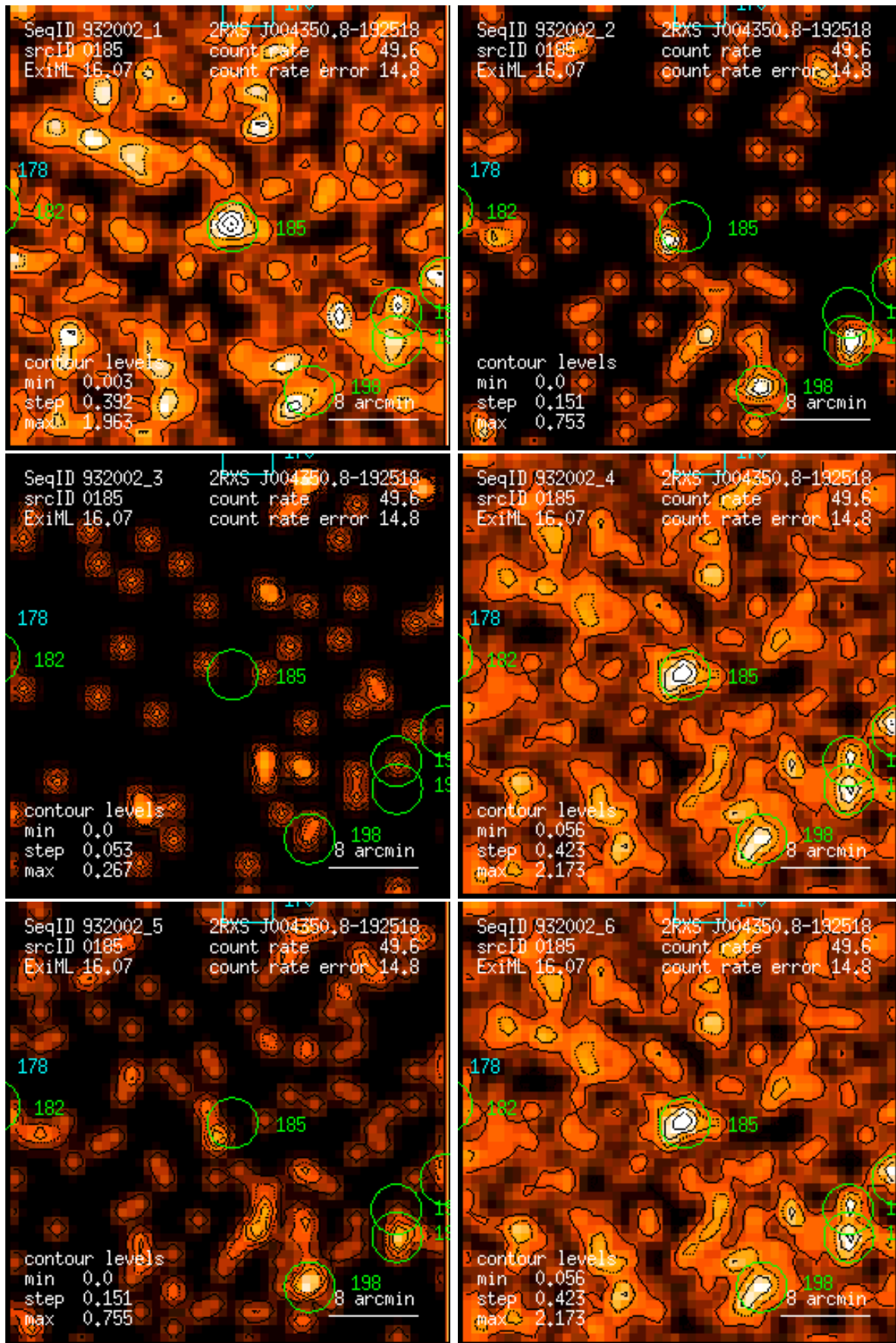
Figure 185: RASS 932002: detection 0185: band rate images, Gaussian filter: (1) PSPC channels 11 – 41, (2) 52 – 90, (3) 91 – 201, (4) 11 – 235, (5) 52 – 201, (6) 11 – 201. Broad band rates in counts/ks. Band rate contour levels in counts/ks/arcmin 2 .
