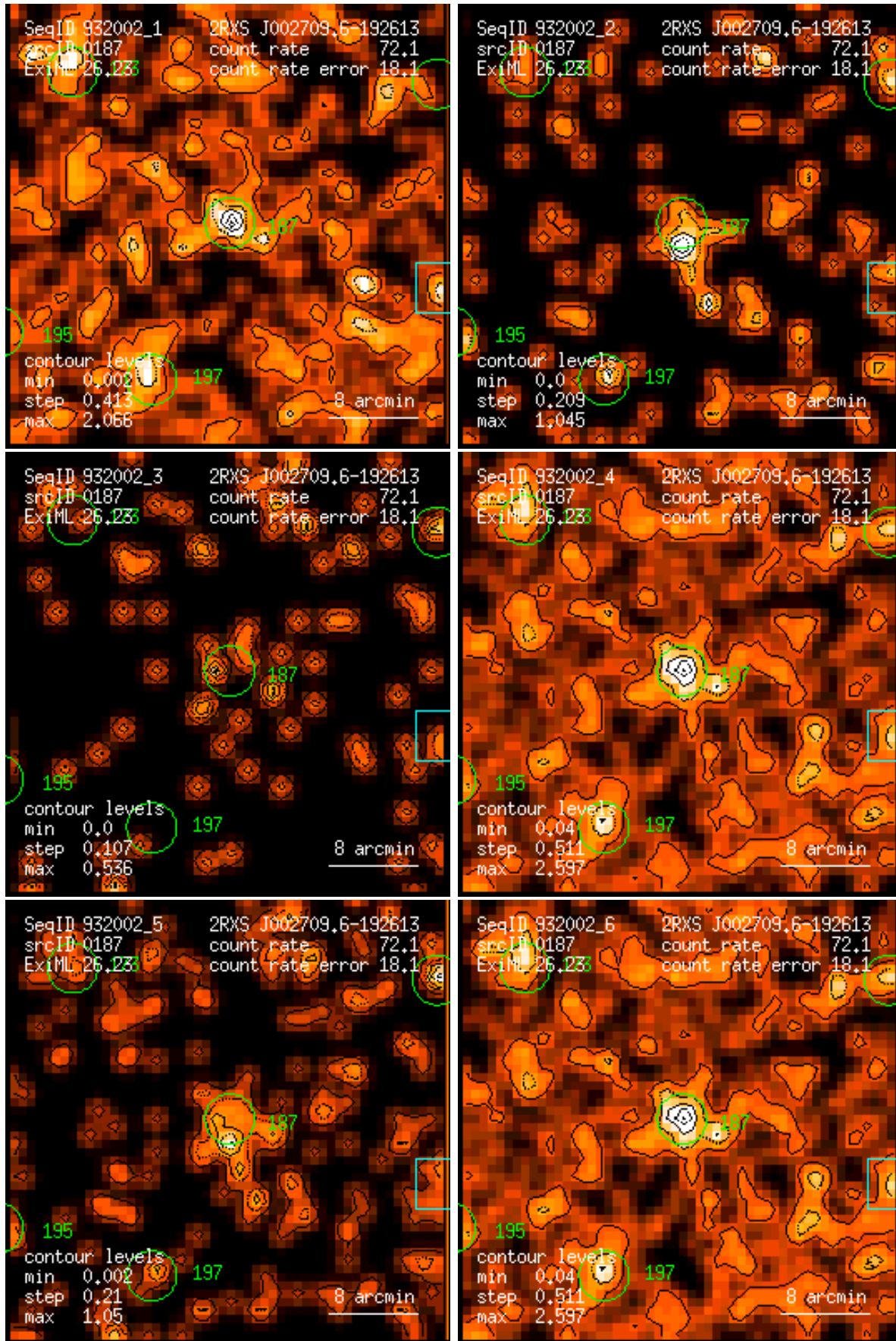
Figure 187: RASS 932002: detection 0187: band rate images, Gaussian filter: (1) PSPC channels 11 – 41, (2) 52 – 90, (3) 91 – 201, (4) 11 – 235, (5) 52 – 201, (6) 11 – 201. Broad band rates in counts/ks. Band rate contour levels in counts/ks/arcmin 2 .
