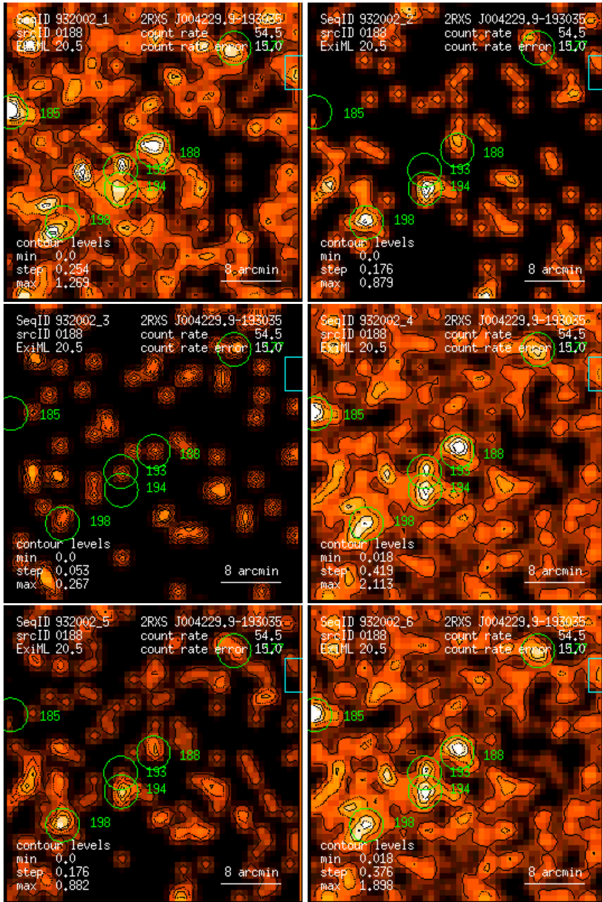
Figure 188: RASS 932002: detection 0188: band rate images, Gaussian filter: (1) PSPC channels 11 – 41, (2) 52 – 90, (3) 91 – 201, (4) 11 – 235, (5) 52 – 201, (6) 11 – 201. Broad band rates in counts/ks. Band rate contour levels in counts/ks/arcmin 2 .
