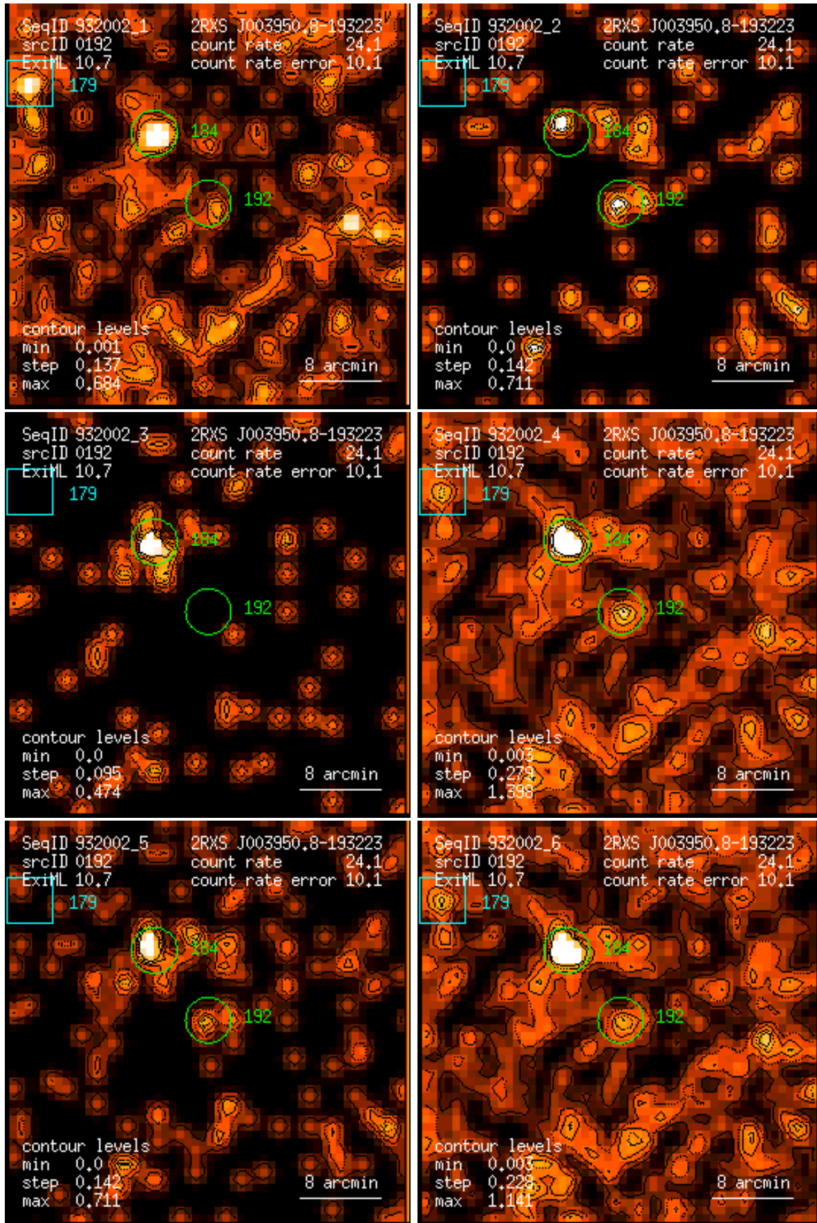
Figure 192: RASS 932002: detection 0192: band rate images, Gaussian filter: (1) PSPC channels 11 – 41, (2) 52 – 90, (3) 91 – 201, (4) 11 – 235, (5) 52 – 201, (6) 11 – 201. Broad band rates in counts/ks. Band rate contour levels in counts/ks/arcmin 2 .
