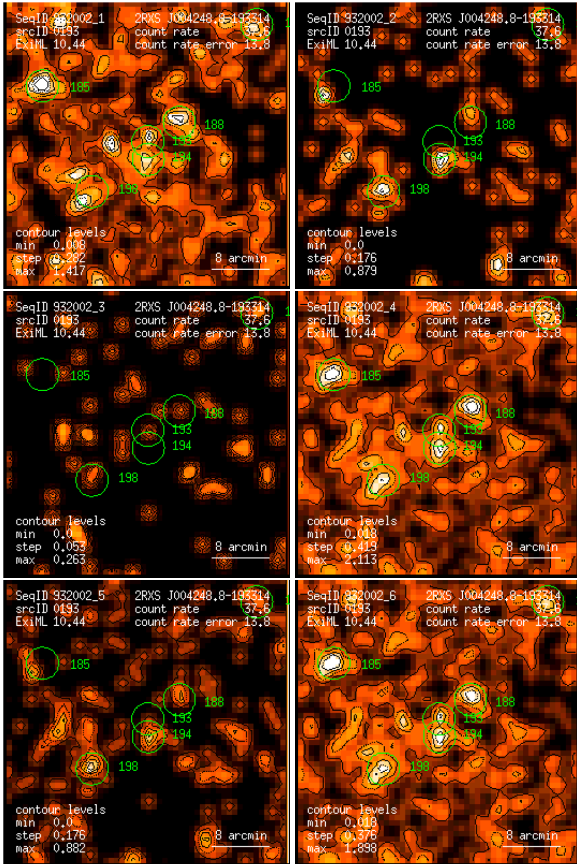
Figure 193: RASS 932002: detection 0193: band rate images, Gaussian filter: (1) PSPC channels 11 – 41, (2) 52 – 90, (3) 91 – 201, (4) 11 – 235, (5) 52 – 201, (6) 11 – 201. Broad band rates in counts/ks. Band rate contour levels in counts/ks/arcmin 2 .
