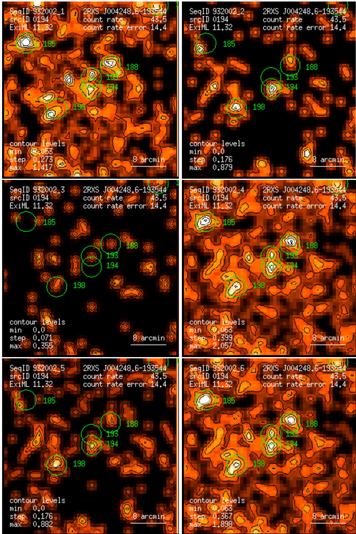
Figure 194: RASS 932002: detection 0194: band rate images, Gaussian filter: (1) PSPC channels 11 – 41, (2) 52 – 90, (3) 91 – 201, (4) 11 – 235, (5) 52 – 201, (6) 11 – 201. Broad band rates in counts/ks. Band rate contour levels in counts/ks/arcmin 2 .
