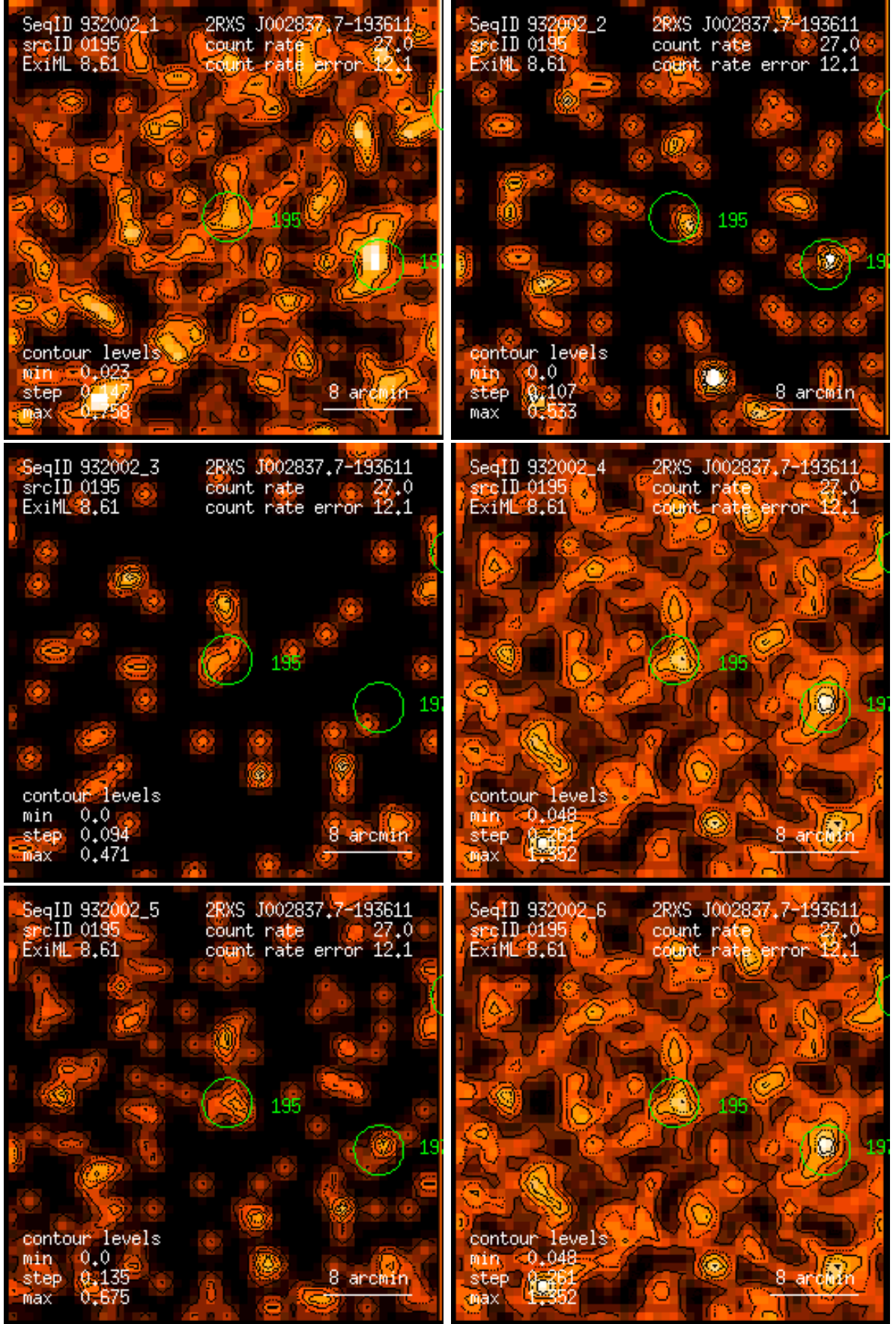
Figure 195: RASS 932002: detection 0195: band rate images, Gaussian filter: (1) PSPC channels 11 – 41, (2) 52 – 90, (3) 91 – 201, (4) 11 – 235, (5) 52 – 201, (6) 11 – 201. Broad band rates in counts/ks. Band rate contour levels in counts/ks/arcmin 2 .
