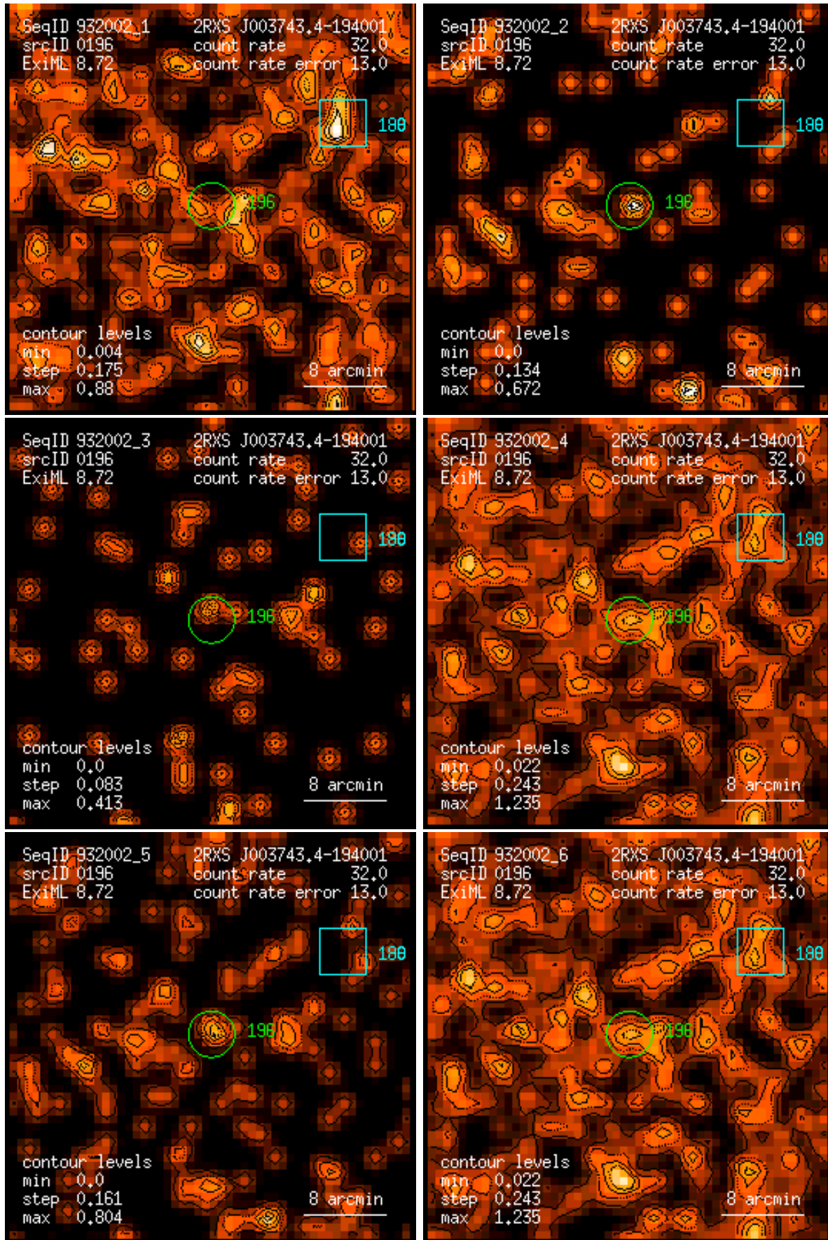
Figure 196: RASS 932002: detection 0196: band rate images, Gaussian filter: (1) PSPC channels 11 – 41, (2) 52 – 90, (3) 91 – 201, (4) 11 – 235, (5) 52 – 201, (6) 11 – 201. Broad band rates in counts/ks. Band rate contour levels in counts/ks/arcmin 2 .
