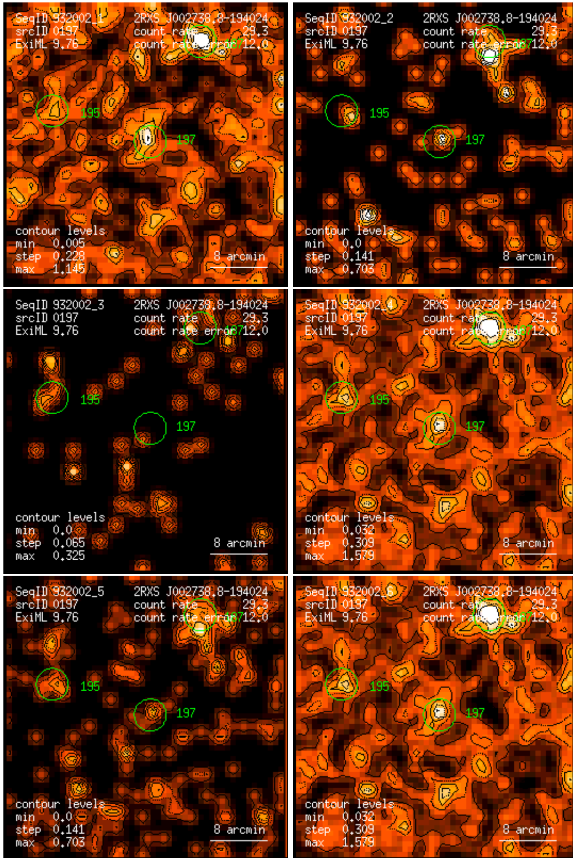
Figure 197: RASS 932002: detection 0197: band rate images, Gaussian filter: (1) PSPC channels 11 – 41, (2) 52 – 90, (3) 91 – 201, (4) 11 – 235, (5) 52 – 201, (6) 11 – 201. Broad band rates in counts/ks. Band rate contour levels in counts/ks/arcmin 2 .
