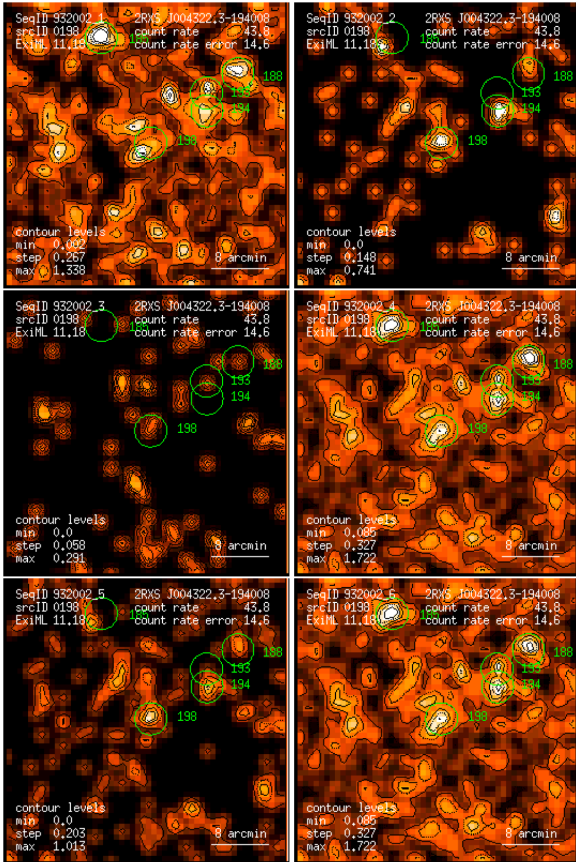
Figure 198: RASS 932002: detection 0198: band rate images, Gaussian filter: (1) PSPC channels 11 – 41, (2) 52 – 90, (3) 91 – 201, (4) 11 – 235, (5) 52 – 201, (6) 11 – 201. Broad band rates in counts/ks. Band rate contour levels in counts/ks/arcmin 2 .
