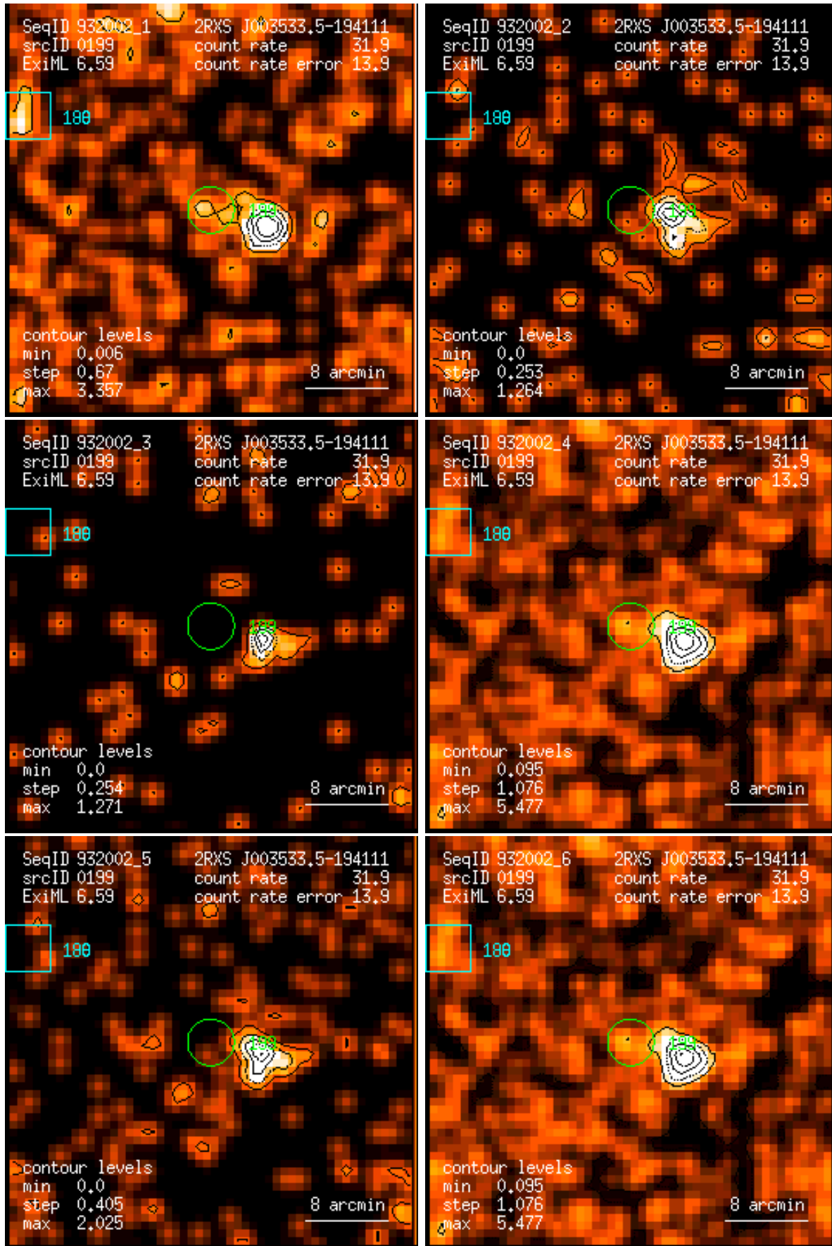
Figure 199: RASS 932002: detection 0199: band rate images, Gaussian filter: (1) PSPC channels 11 – 41, (2) 52 – 90, (3) 91 – 201, (4) 11 – 235, (5) 52 – 201, (6) 11 – 201. Broad band rates in counts/ks. Band rate contour levels in counts/ks/arcmin 2 .
