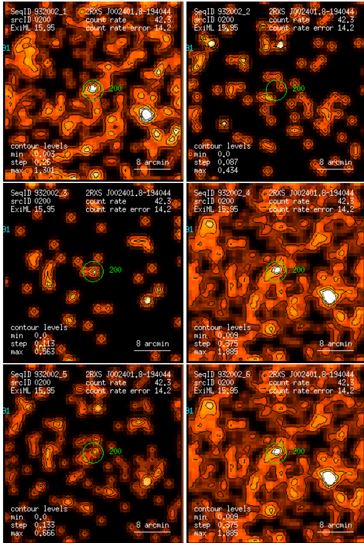
Figure 200: RASS 932002: detection 0200: band rate images, Gaussian filter: (1) PSPC channels 11 – 41, (2) 52 – 90, (3) 91 – 201, (4) 11 – 235, (5) 52 – 201, (6) 11 – 201. Broad band rates in counts/ks. Band rate contour levels in counts/ks/arcmin 2 .
