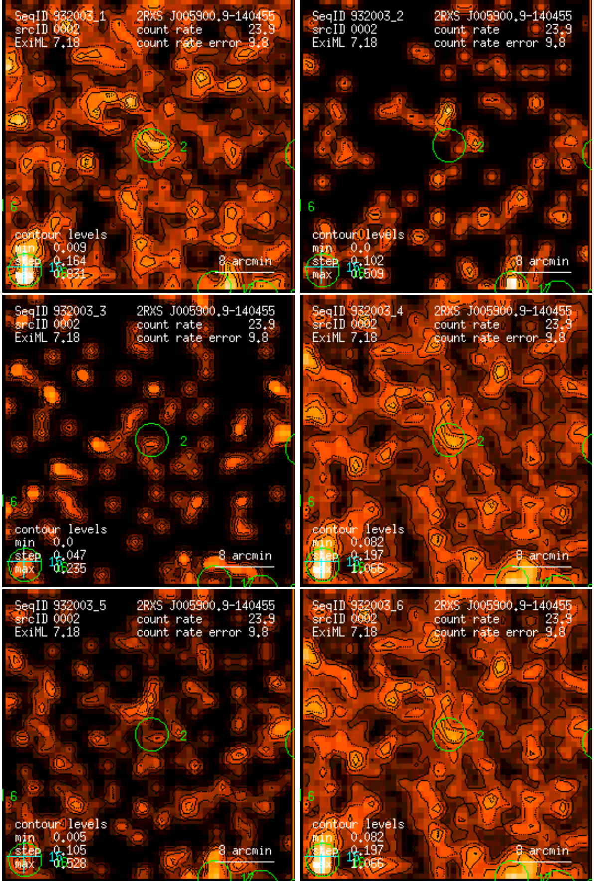
Figure 2: RASS 932003: detection 0002: band rate images, Gaussian filter: (1) PSPC channels 11 – 41, (2) 52 – 90, (3) 91 – 201, (4) 11 – 235, (5) 52 – 201, (6) 11 – 201. Broad band rates in counts/ks. Band rate contour levels in counts/ks/arcmin 2 .
