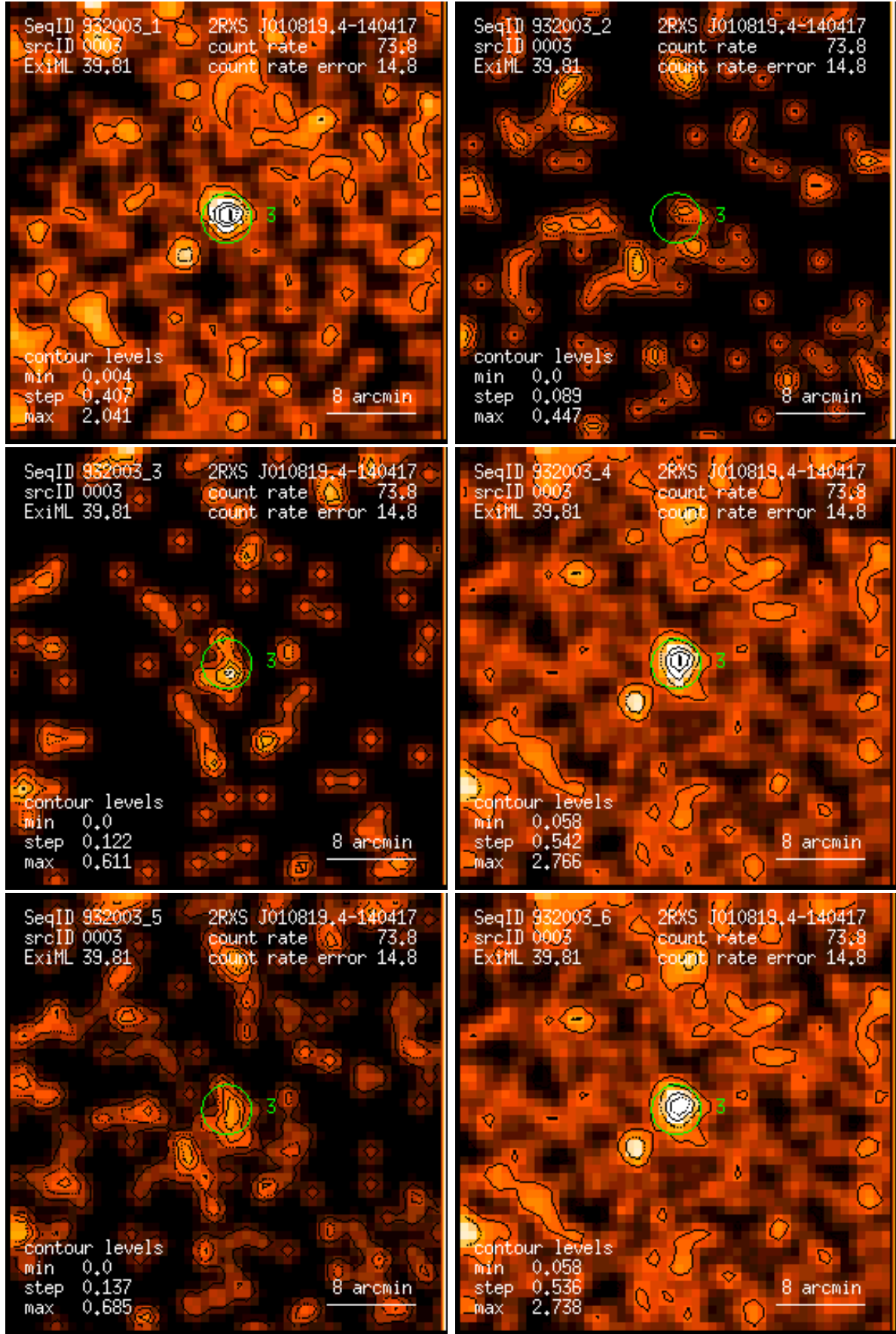
Figure 3: RASS 932003: detection 0003: band rate images, Gaussian filter: (1) PSPC channels 11 – 41, (2) 52 – 90, (3) 91 – 201, (4) 11 – 235, (5) 52 – 201, (6) 11 – 201. Broad band rates in counts/ks. Band rate contour levels in counts/ks/arcmin 2 .
