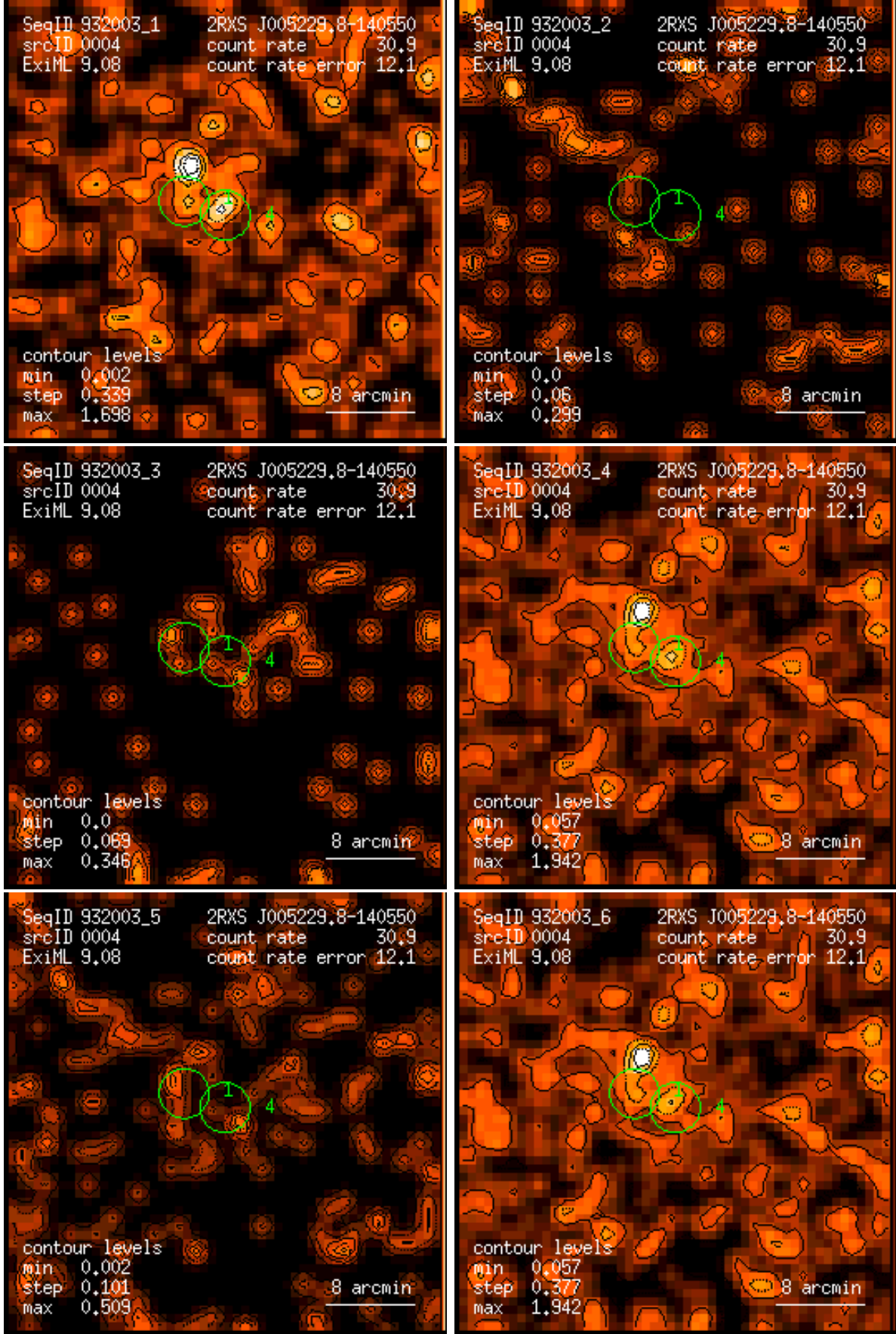
Figure 4: RASS 932003: detection 0004: band rate images, Gaussian filter: (1) PSPC channels 11 – 41, (2) 52 – 90, (3) 91 – 201, (4) 11 – 235, (5) 52 – 201, (6) 11 – 201. Broad band rates in counts/ks. Band rate contour levels in counts/ks/arcmin 2 .
