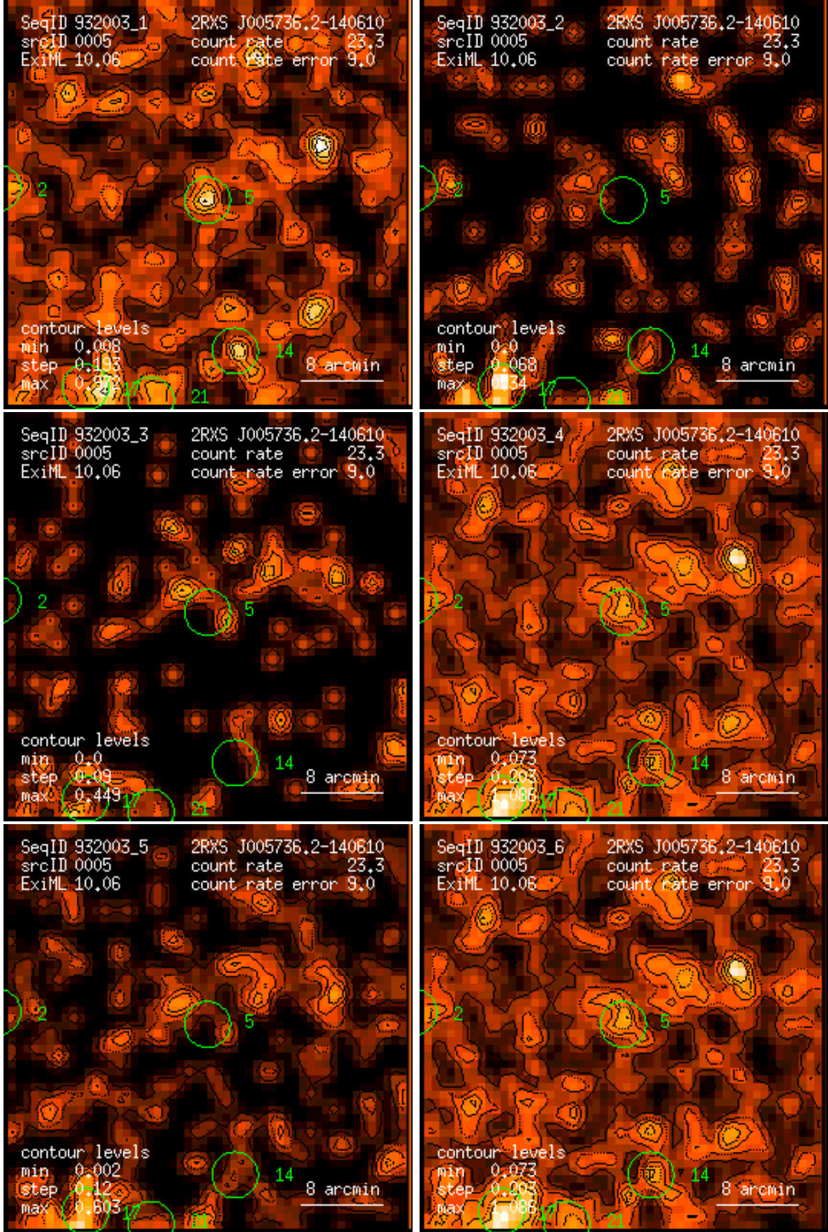
Figure 5: RASS 932003: detection 0005: band rate images, Gaussian filter: (1) PSPC channels 11 – 41, (2) 52 – 90, (3) 91 – 201, (4) 11 – 235, (5) 52 – 201, (6) 11 – 201. Broad band rates in counts/ks. Band rate contour levels in counts/ks/arcmin 2 .
