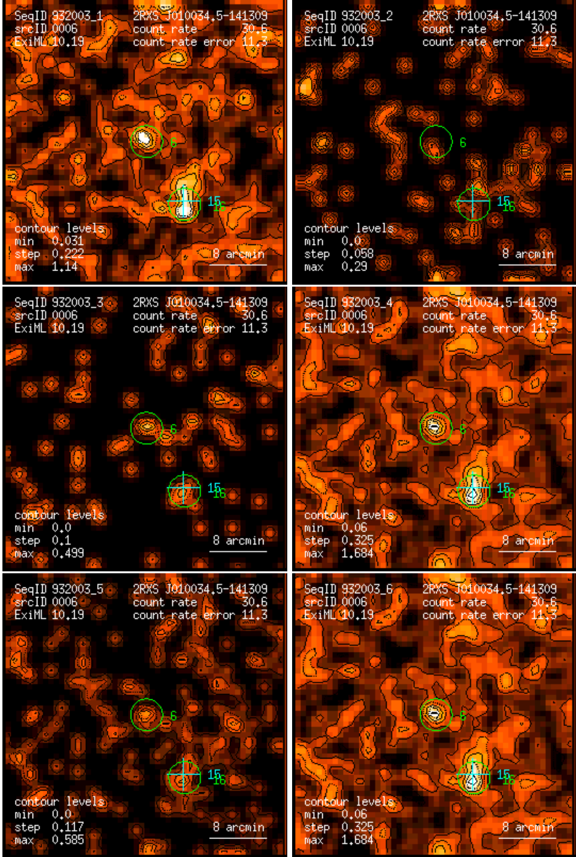
Figure 6: RASS 932003: detection 0006: band rate images, Gaussian filter: (1) PSPC channels 11 – 41, (2) 52 – 90, (3) 91 – 201, (4) 11 – 235, (5) 52 – 201, (6) 11 – 201. Broad band rates in counts/ks. Band rate contour levels in counts/ks/arcmin 2 .
