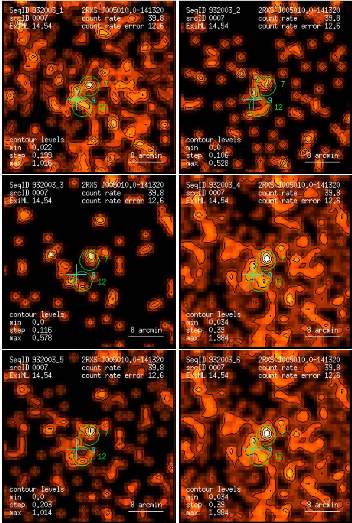
Figure 7: RASS 932003: detection 0007: band rate images, Gaussian filter: (1) PSPC channels 11 – 41, (2) 52 – 90, (3) 91 – 201, (4) 11 – 235, (5) 52 – 201, (6) 11 – 201. Broad band rates in counts/ks. Band rate contour levels in counts/ks/arcmin 2 .
