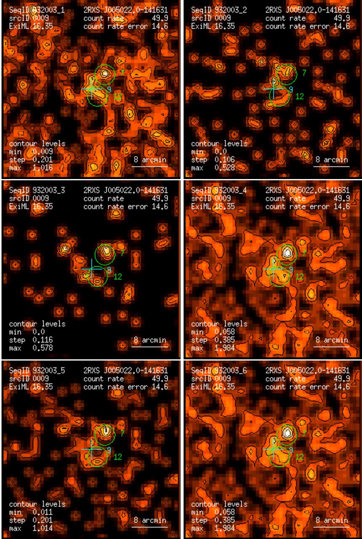
Figure 9: RASS 932003: detection 0009: band rate images, Gaussian filter: (1) PSPC channels 11 – 41, (2) 52 – 90, (3) 91 – 201, (4) 11 – 235, (5) 52 – 201, (6) 11 – 201. Broad band rates in counts/ks. Band rate contour levels in counts/ks/arcmin 2 .
