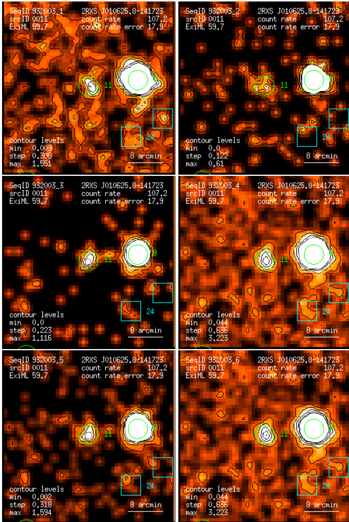
Figure 11: RASS 932003: detection 0011: band rate images, Gaussian filter: (1) PSPC channels 11 – 41, (2) 52 – 90, (3) 91 – 201, (4) 11 – 235, (5) 52 – 201, (6) 11 – 201. Broad band rates in counts/ks. Band rate contour levels in counts/ks/arcmin 2 .
