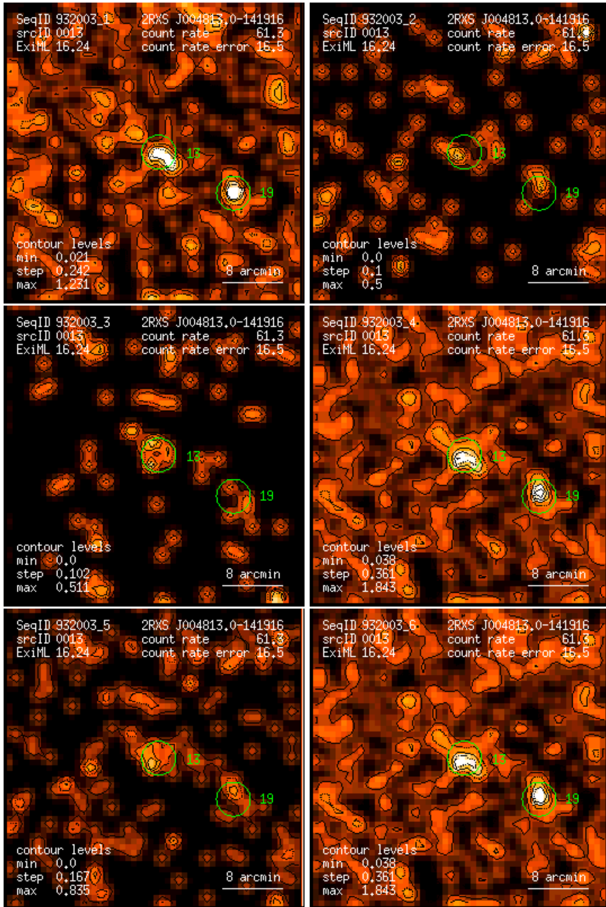
Figure 13: RASS 932003: detection 0013: band rate images, Gaussian filter: (1) PSPC channels 11 – 41, (2) 52 – 90, (3) 91 – 201, (4) 11 – 235, (5) 52 – 201, (6) 11 – 201. Broad band rates in counts/ks. Band rate contour levels in counts/ks/arcmin 2 .
