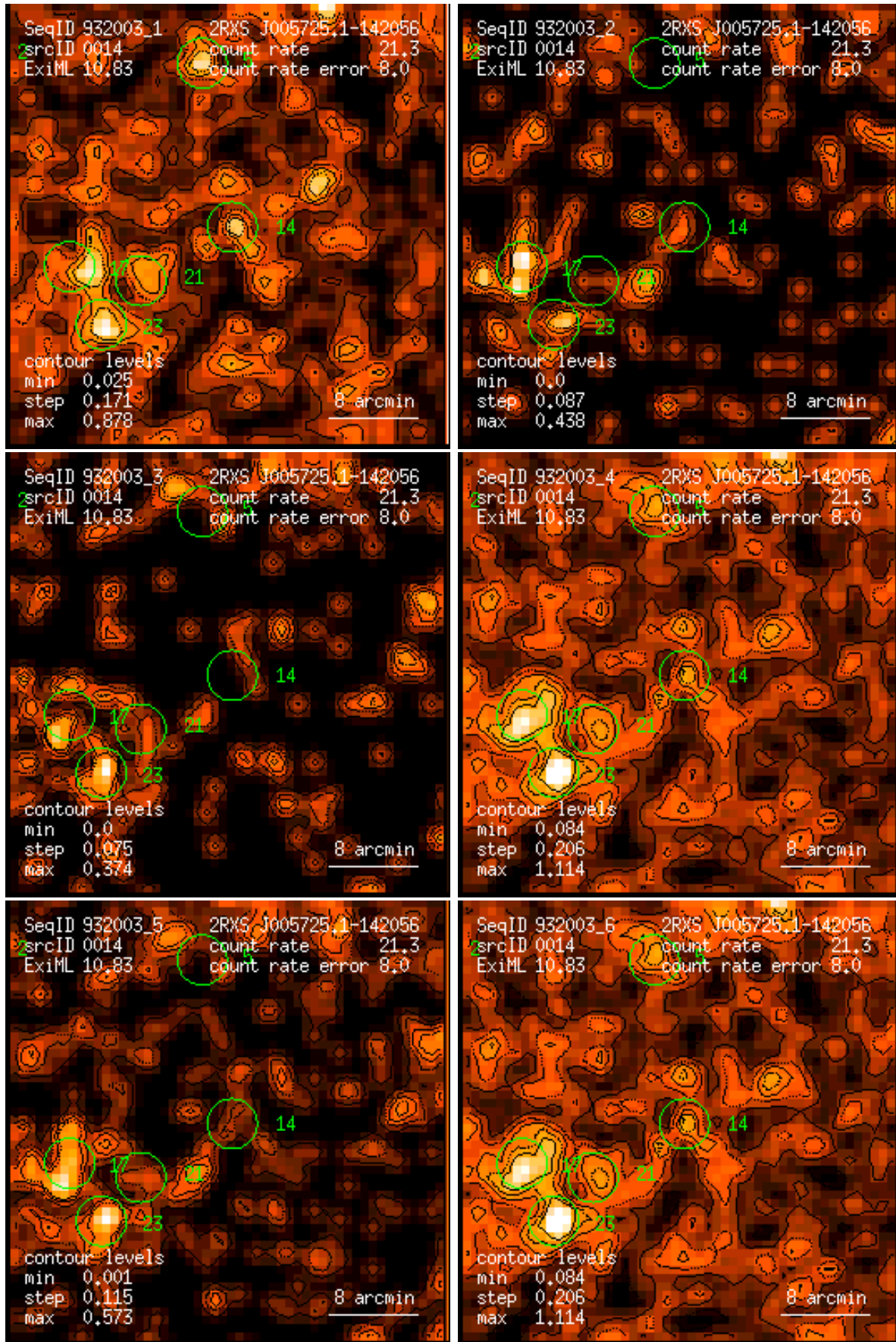
Figure 14: RASS 932003: detection 0014: band rate images, Gaussian filter: (1) PSPC channels 11 – 41, (2) 52 – 90, (3) 91 – 201, (4) 11 – 235, (5) 52 – 201, (6) 11 – 201. Broad band rates in counts/ks. Band rate contour levels in counts/ks/arcmin 2 .
