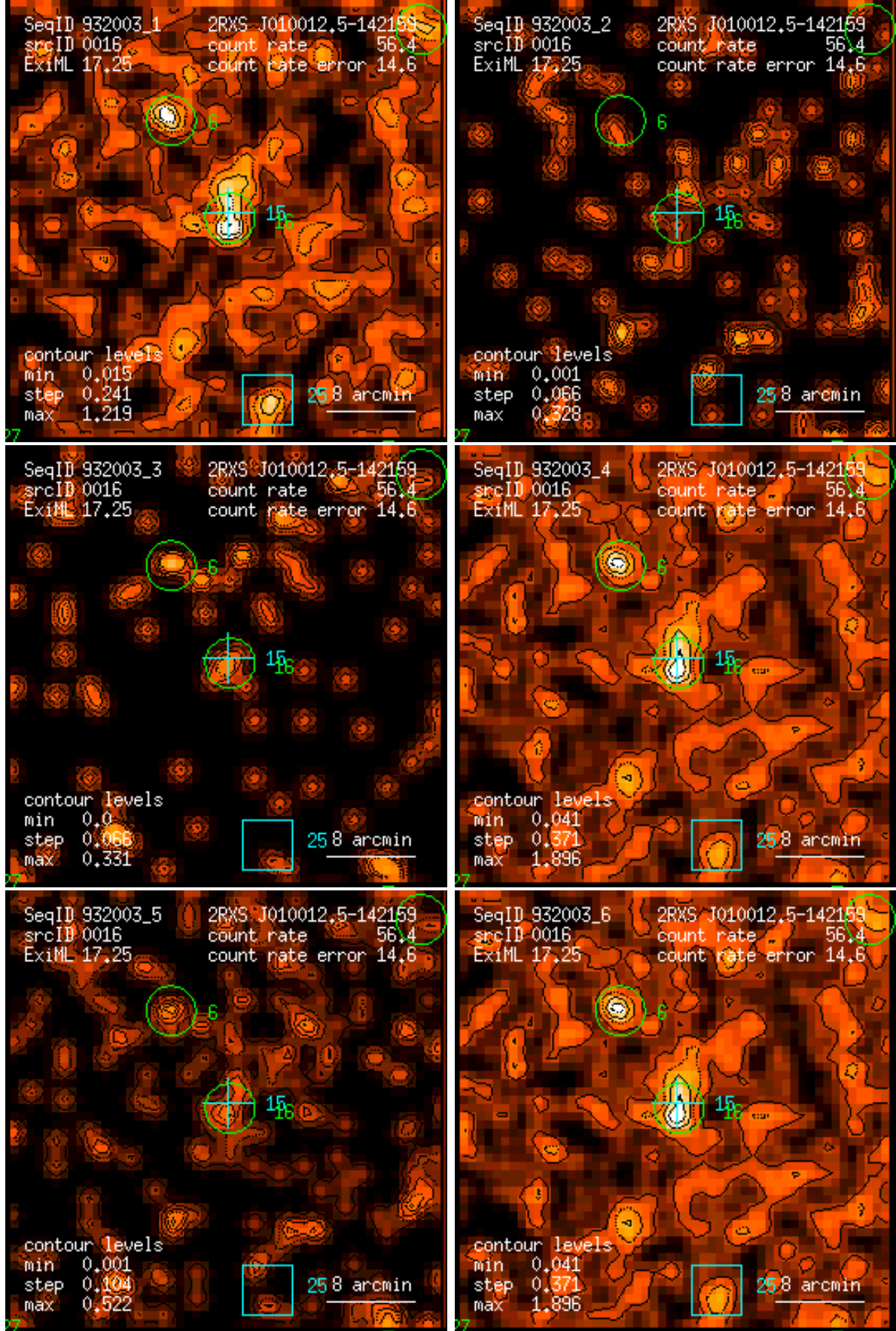
Figure 16: RASS 932003: detection 0016: band rate images, Gaussian filter: (1) PSPC channels 11 – 41, (2) 52 – 90, (3) 91 – 201, (4) 11 – 235, (5) 52 – 201, (6) 11 – 201. Broad band rates in counts/ks. Band rate contour levels in counts/ks/arcmin 2 .
