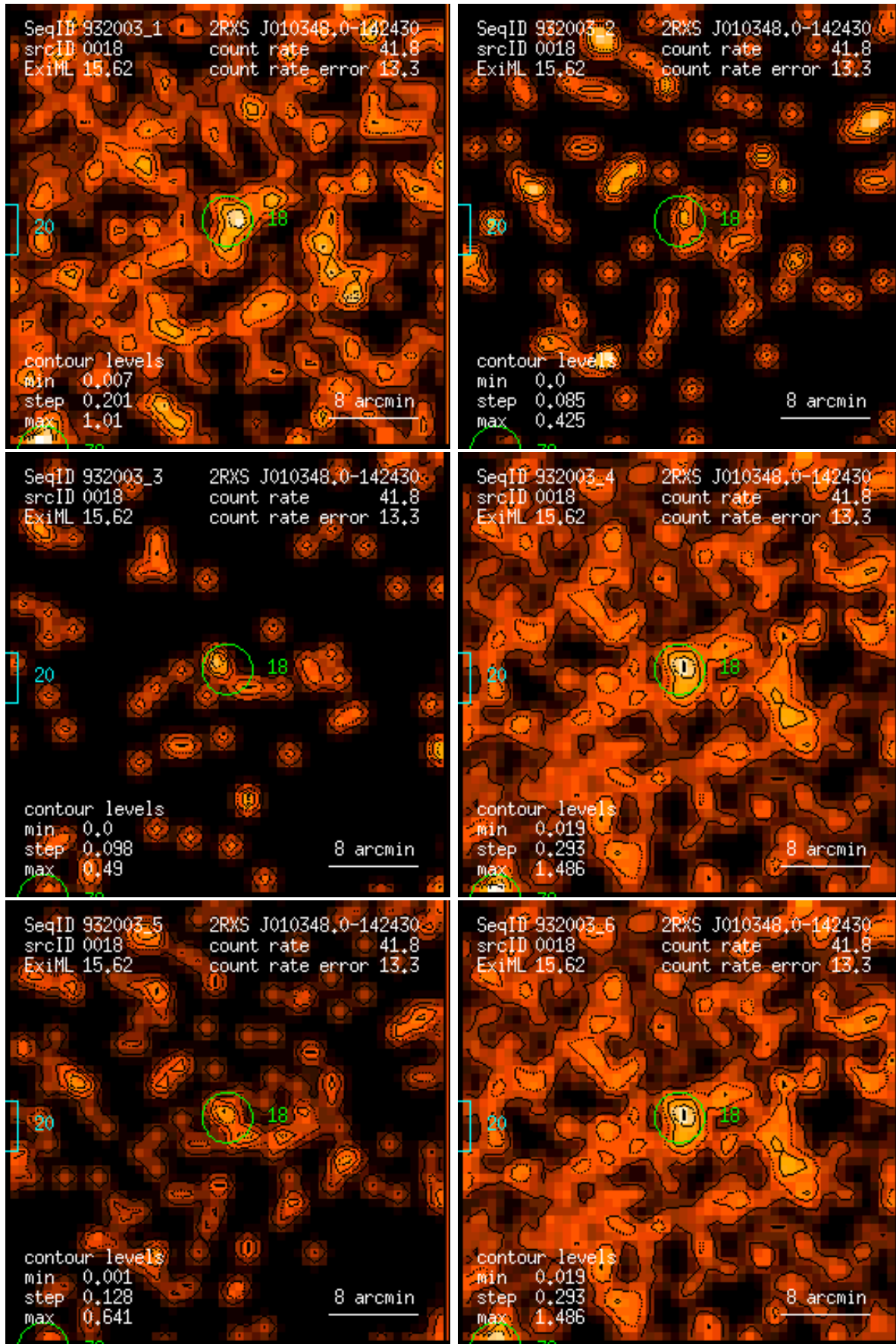
Figure 18: RASS 932003: detection 0018: band rate images, Gaussian filter: (1) PSPC channels 11 – 41, (2) 52 – 90, (3) 91 – 201, (4) 11 – 235, (5) 52 – 201, (6) 11 – 201. Broad band rates in counts/ks. Band rate contour levels in counts/ks/arcmin 2 .
