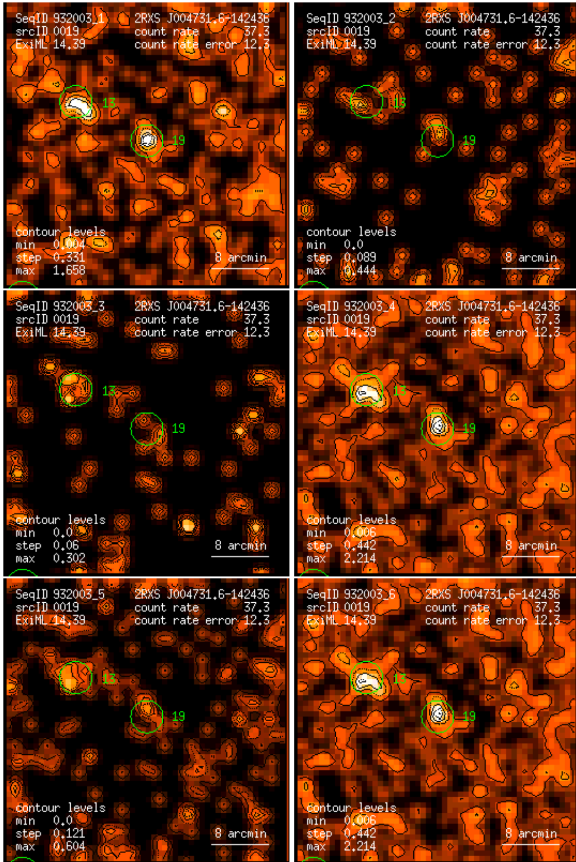
Figure 19: RASS 932003: detection 0019: band rate images, Gaussian filter: (1) PSPC channels 11 – 41, (2) 52 – 90, (3) 91 – 201, (4) 11 – 235, (5) 52 – 201, (6) 11 – 201. Broad band rates in counts/ks. Band rate contour levels in counts/ks/arcmin 2 .
