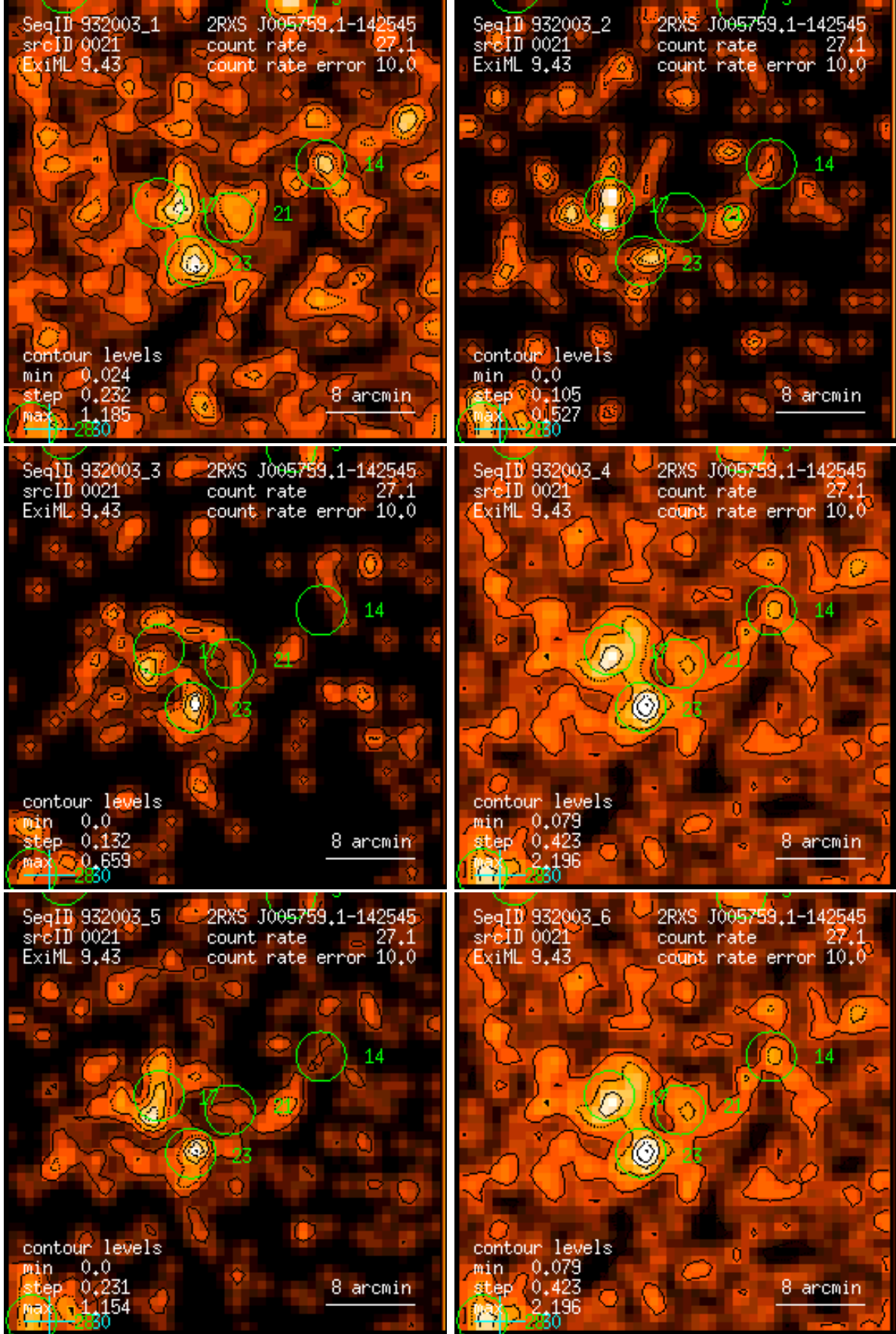
Figure 21: RASS 932003: detection 0021: band rate images, Gaussian filter: (1) PSPC channels 11 – 41, (2) 52 – 90, (3) 91 – 201, (4) 11 – 235, (5) 52 – 201, (6) 11 – 201. Broad band rates in counts/ks. Band rate contour levels in counts/ks/arcmin 2 .
