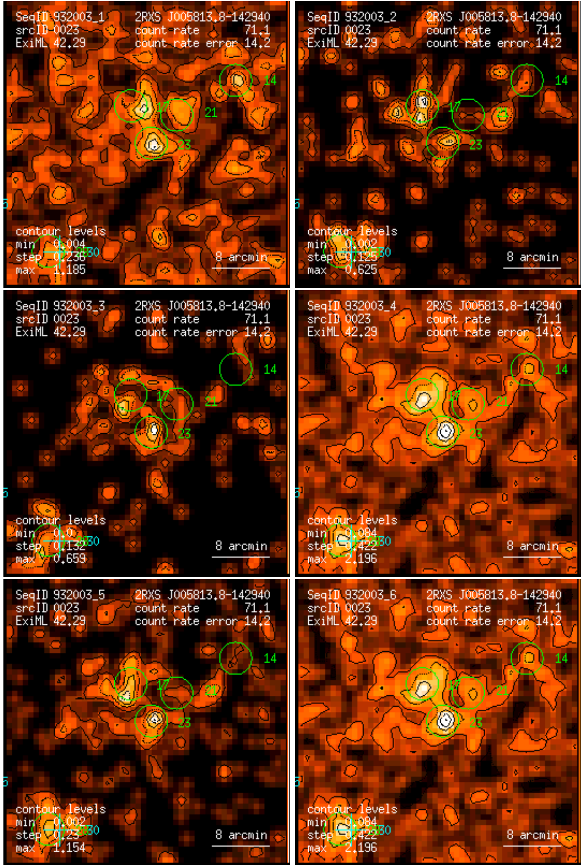
Figure 23: RASS 932003: detection 0023: band rate images, Gaussian filter: (1) PSPC channels 11 – 41, (2) 52 – 90, (3) 91 – 201, (4) 11 – 235, (5) 52 – 201, (6) 11 – 201. Broad band rates in counts/ks. Band rate contour levels in counts/ks/arcmin 2 .
