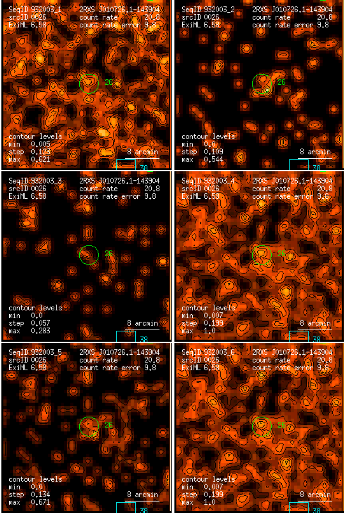
Figure 26: RASS 932003: detection 0026: band rate images, Gaussian filter: (1) PSPC channels 11 – 41, (2) 52 – 90, (3) 91 – 201, (4) 11 – 235, (5) 52 – 201, (6) 11 – 201. Broad band rates in counts/ks. Band rate contour levels in counts/ks/arcmin 2 .
