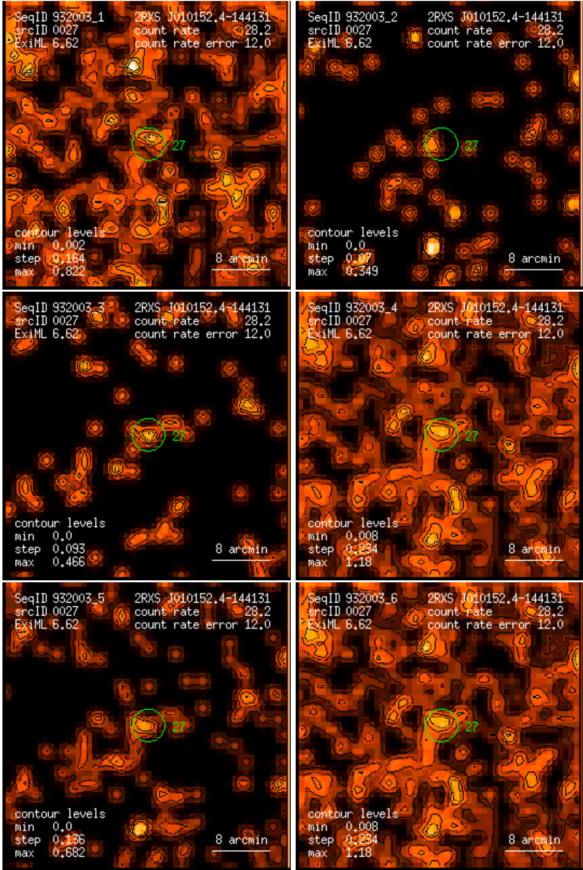
Figure 27: RASS 932003: detection 0027: band rate images, Gaussian filter: (1) PSPC channels 11 – 41, (2) 52 – 90, (3) 91 – 201, (4) 11 – 235, (5) 52 – 201, (6) 11 – 201. Broad band rates in counts/ks. Band rate contour levels in counts/ks/arcmin 2 .
