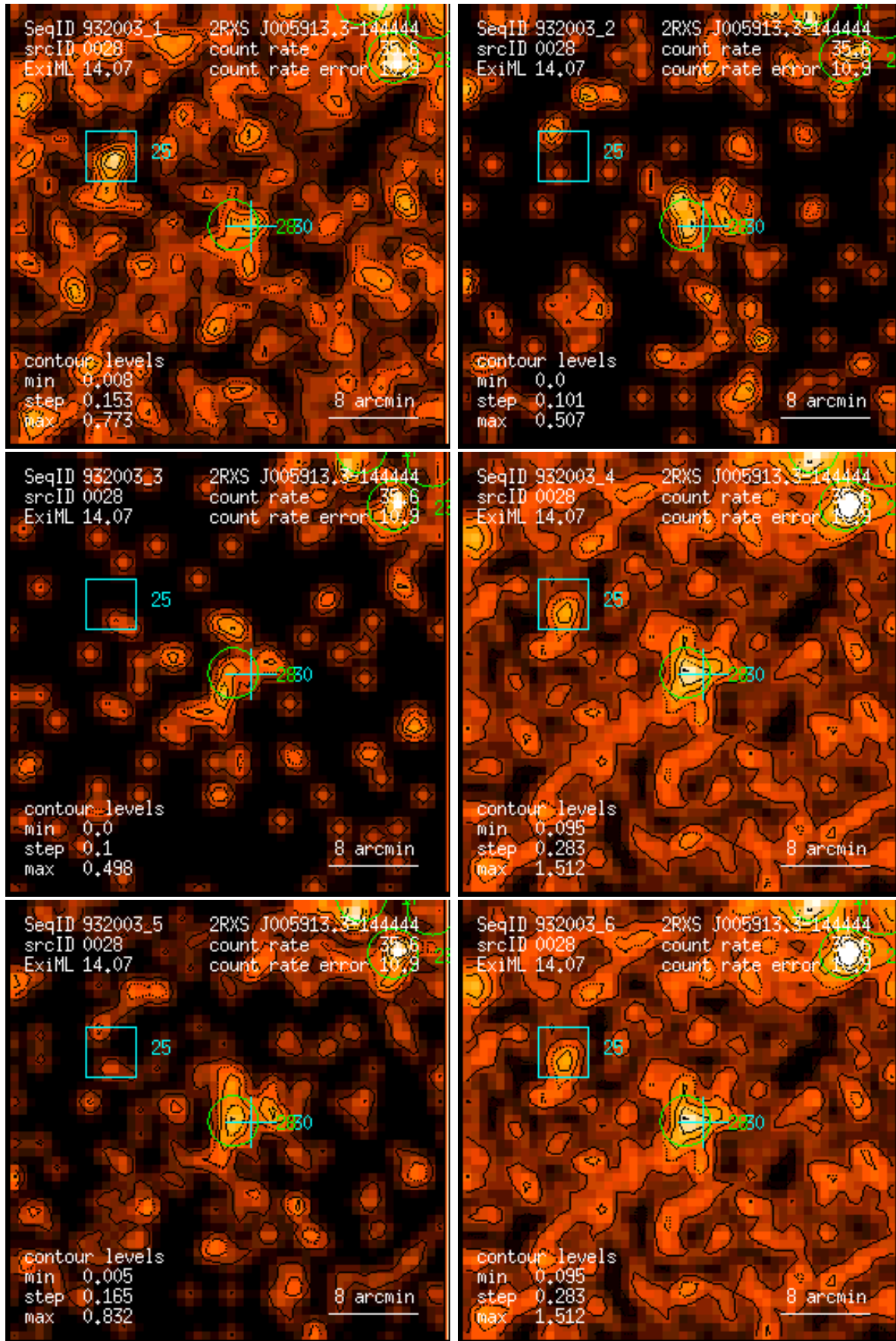
Figure 28: RASS 932003: detection 0028: band rate images, Gaussian filter: (1) PSPC channels 11 – 41, (2) 52 – 90, (3) 91 – 201, (4) 11 – 235, (5) 52 – 201, (6) 11 – 201. Broad band rates in counts/ks. Band rate contour levels in counts/ks/arcmin 2 .
