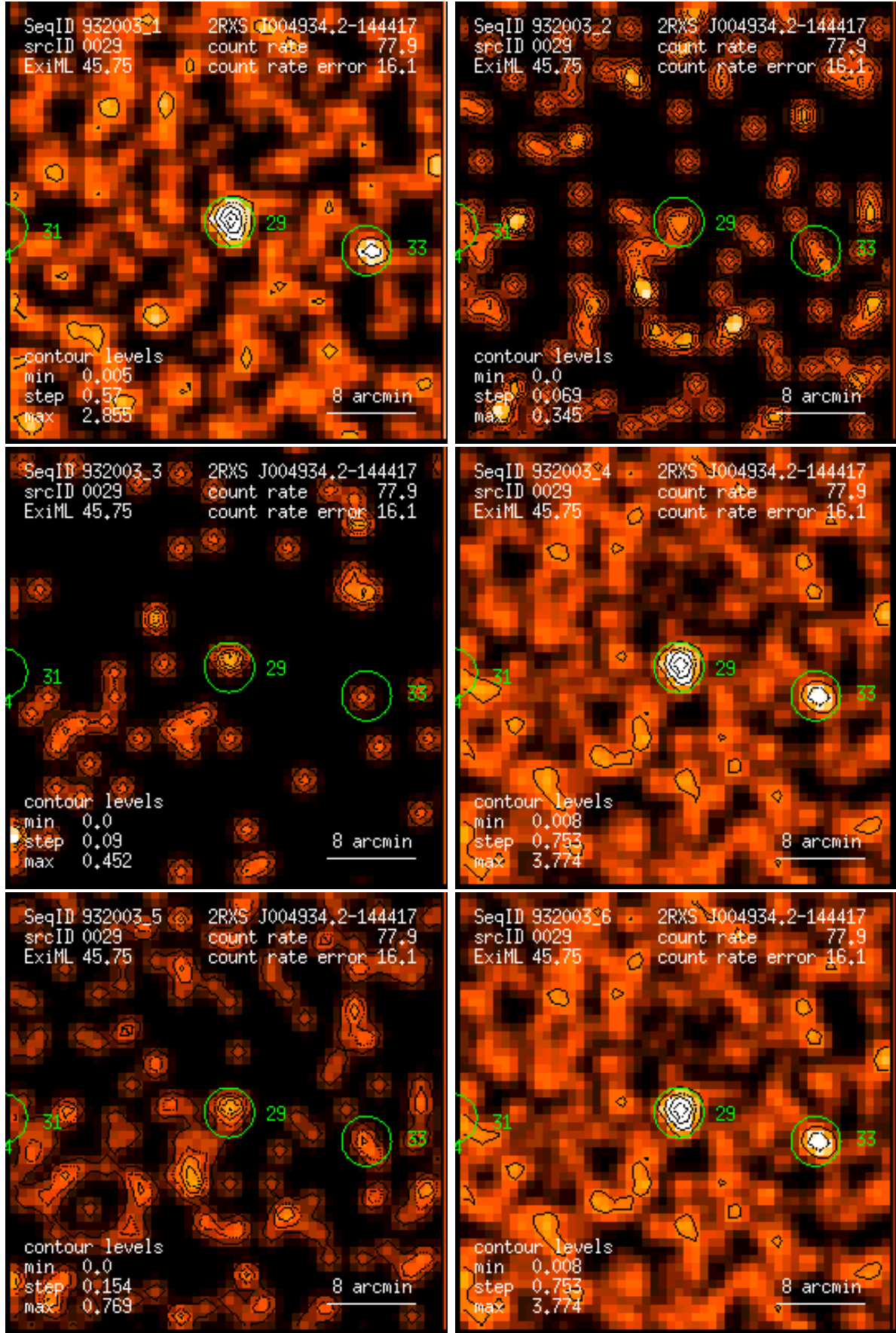
Figure 29: RASS 932003: detection 0029: band rate images, Gaussian filter: (1) PSPC channels 11 – 41, (2) 52 – 90, (3) 91 – 201, (4) 11 – 235, (5) 52 – 201, (6) 11 – 201. Broad band rates in counts/ks. Band rate contour levels in counts/ks/arcmin 2 .
