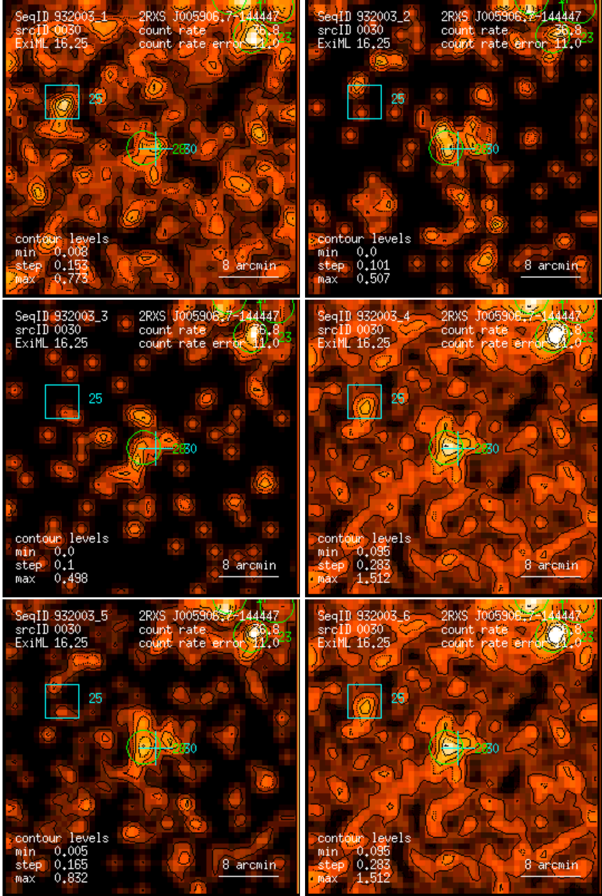
Figure 30: RASS 932003: detection 0030: band rate images, Gaussian filter: (1) PSPC channels 11 – 41, (2) 52 – 90, (3) 91 – 201, (4) 11 – 235, (5) 52 – 201, (6) 11 – 201. Broad band rates in counts/ks. Band rate contour levels in counts/ks/arcmin 2 .
