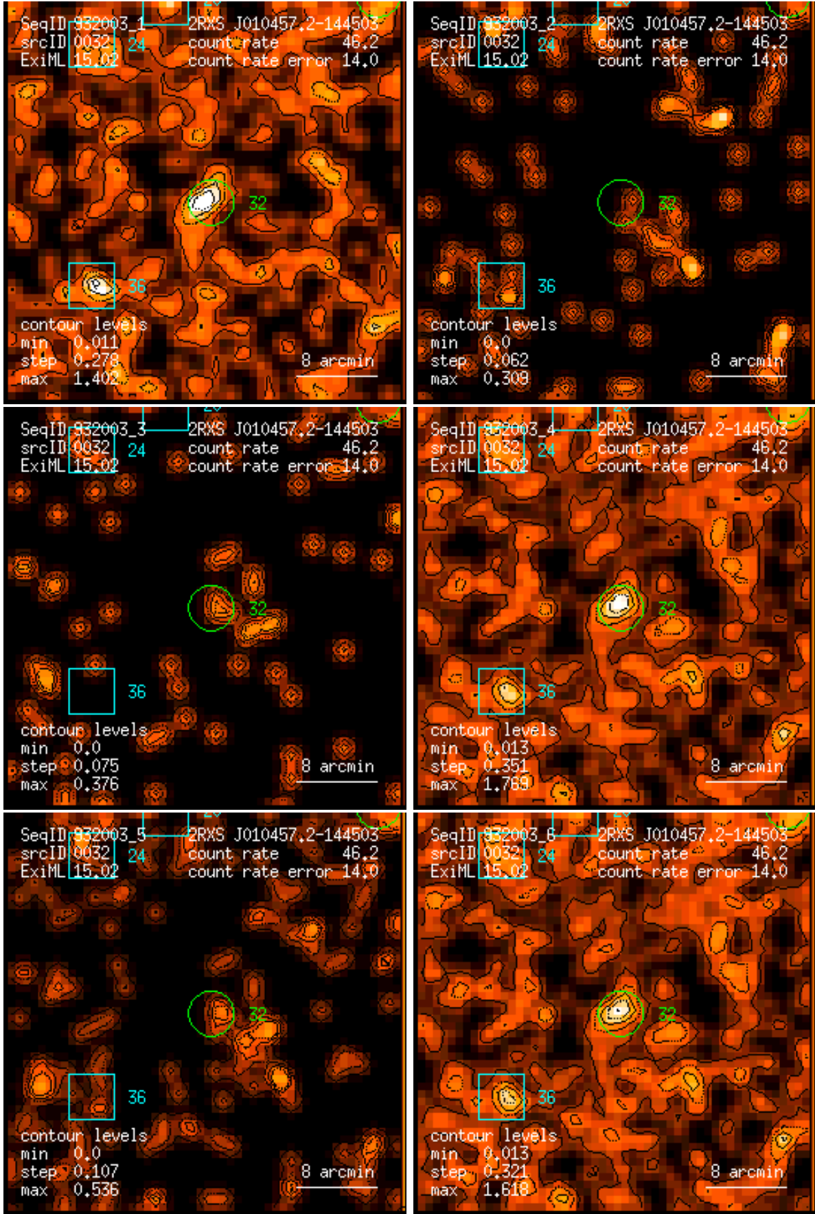
Figure 32: RASS 932003: detection 0032: band rate images, Gaussian filter: (1) PSPC channels 11 – 41, (2) 52 – 90, (3) 91 – 201, (4) 11 – 235, (5) 52 – 201, (6) 11 – 201. Broad band rates in counts/ks. Band rate contour levels in counts/ks/arcmin 2 .
