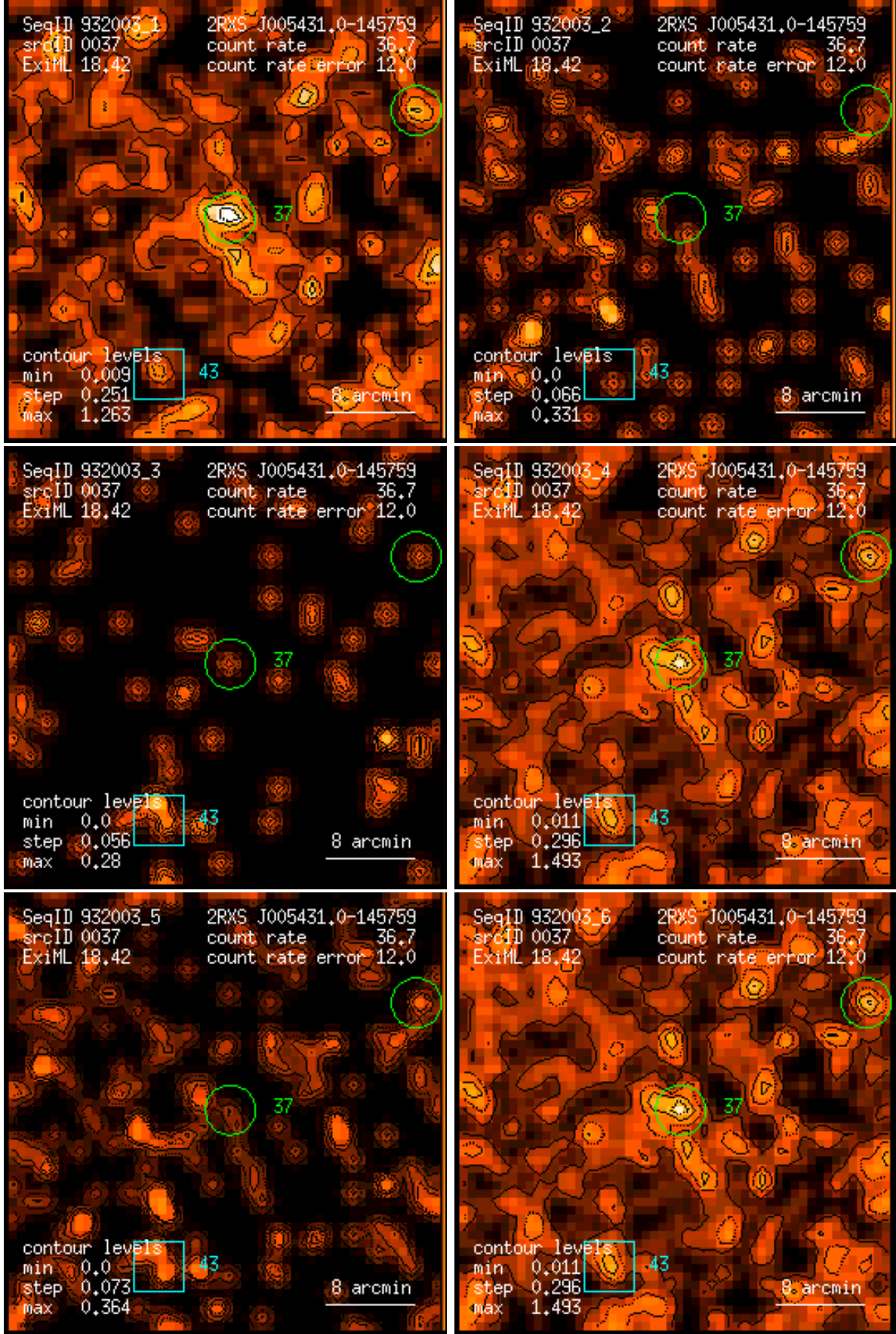
Figure 37: RASS 932003: detection 0037: band rate images, Gaussian filter: (1) PSPC channels 11 – 41, (2) 52 – 90, (3) 91 – 201, (4) 11 – 235, (5) 52 – 201, (6) 11 – 201. Broad band rates in counts/ks. Band rate contour levels in counts/ks/arcmin 2 .
