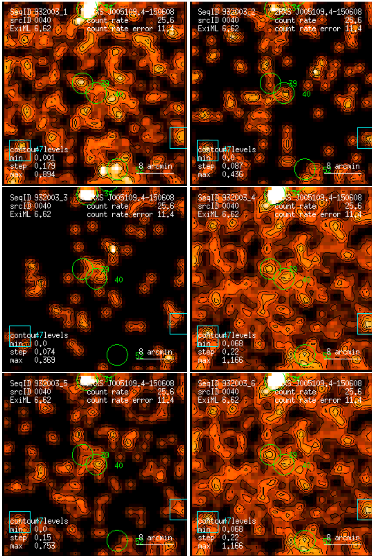
Figure 40: RASS 932003: detection 0040: band rate images, Gaussian filter: (1) PSPC channels 11 – 41, (2) 52 – 90, (3) 91 – 201, (4) 11 – 235, (5) 52 – 201, (6) 11 – 201. Broad band rates in counts/ks. Band rate contour levels in counts/ks/arcmin 2 .
