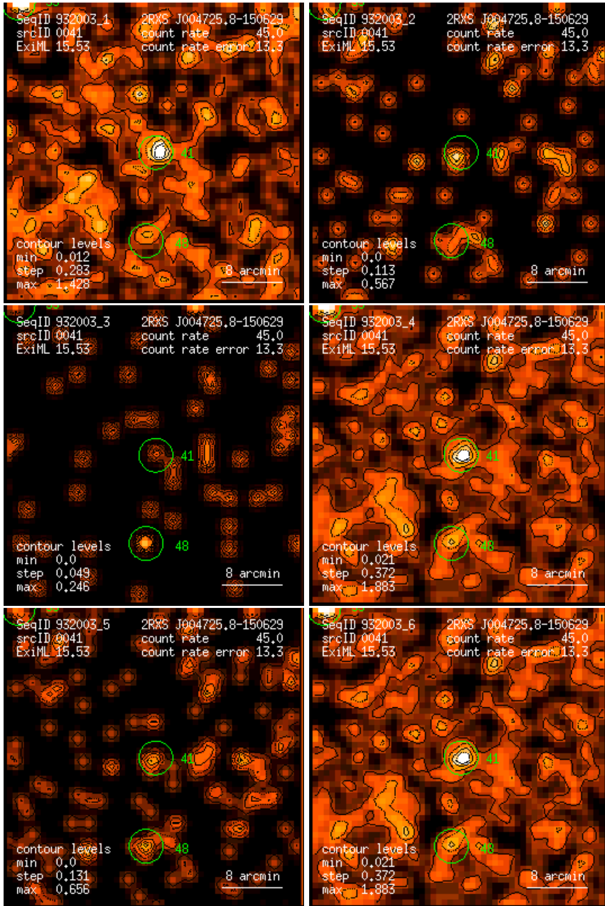
Figure 41: RASS 932003: detection 0041: band rate images, Gaussian filter: (1) PSPC channels 11 – 41, (2) 52 – 90, (3) 91 – 201, (4) 11 – 235, (5) 52 – 201, (6) 11 – 201. Broad band rates in counts/ks. Band rate contour levels in counts/ks/arcmin 2 .
