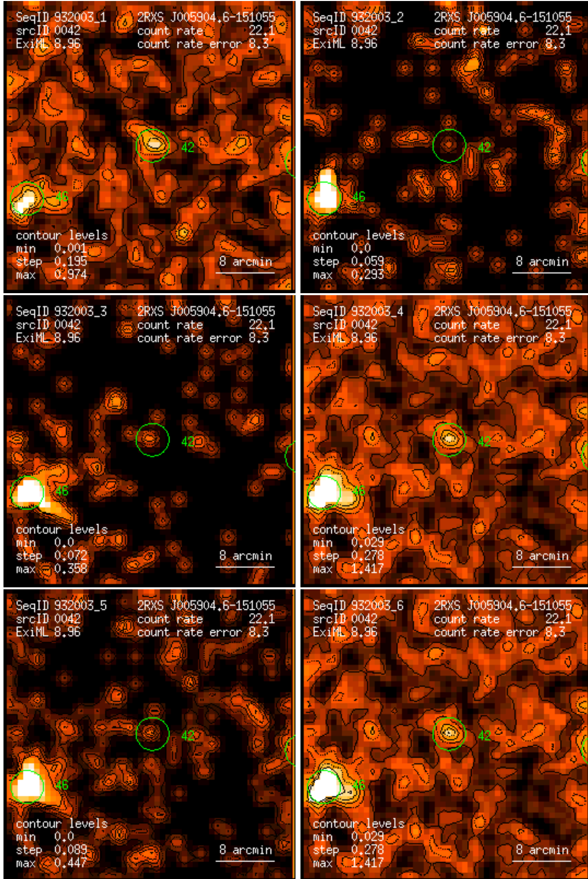
Figure 42: RASS 932003: detection 0042: band rate images, Gaussian filter: (1) PSPC channels 11 – 41, (2) 52 – 90, (3) 91 – 201, (4) 11 – 235, (5) 52 – 201, (6) 11 – 201. Broad band rates in counts/ks. Band rate contour levels in counts/ks/arcmin 2 .
