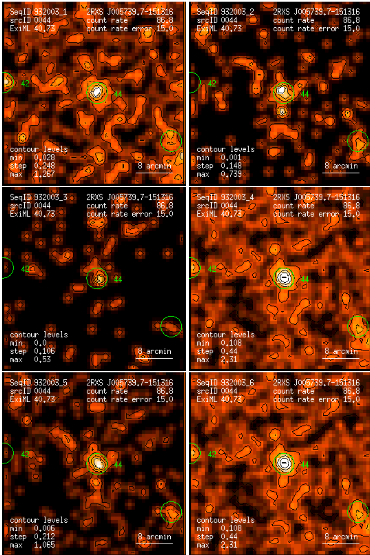
Figure 44: RASS 932003: detection 0044: band rate images, Gaussian filter: (1) PSPC channels 11 – 41, (2) 52 – 90, (3) 91 – 201, (4) 11 – 235, (5) 52 – 201, (6) 11 – 201. Broad band rates in counts/ks. Band rate contour levels in counts/ks/arcmin 2 .
