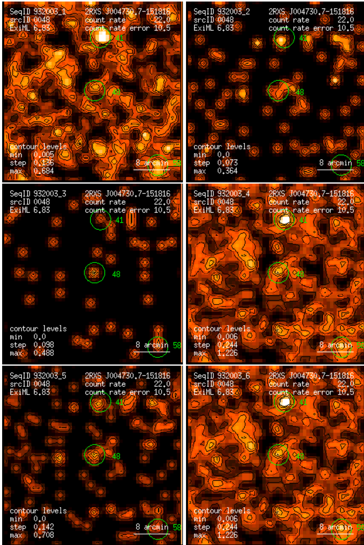
Figure 48: RASS 932003: detection 0048: band rate images, Gaussian filter: (1) PSPC channels 11 – 41, (2) 52 – 90, (3) 91 – 201, (4) 11 – 235, (5) 52 – 201, (6) 11 – 201. Broad band rates in counts/ks. Band rate contour levels in counts/ks/arcmin 2 .
