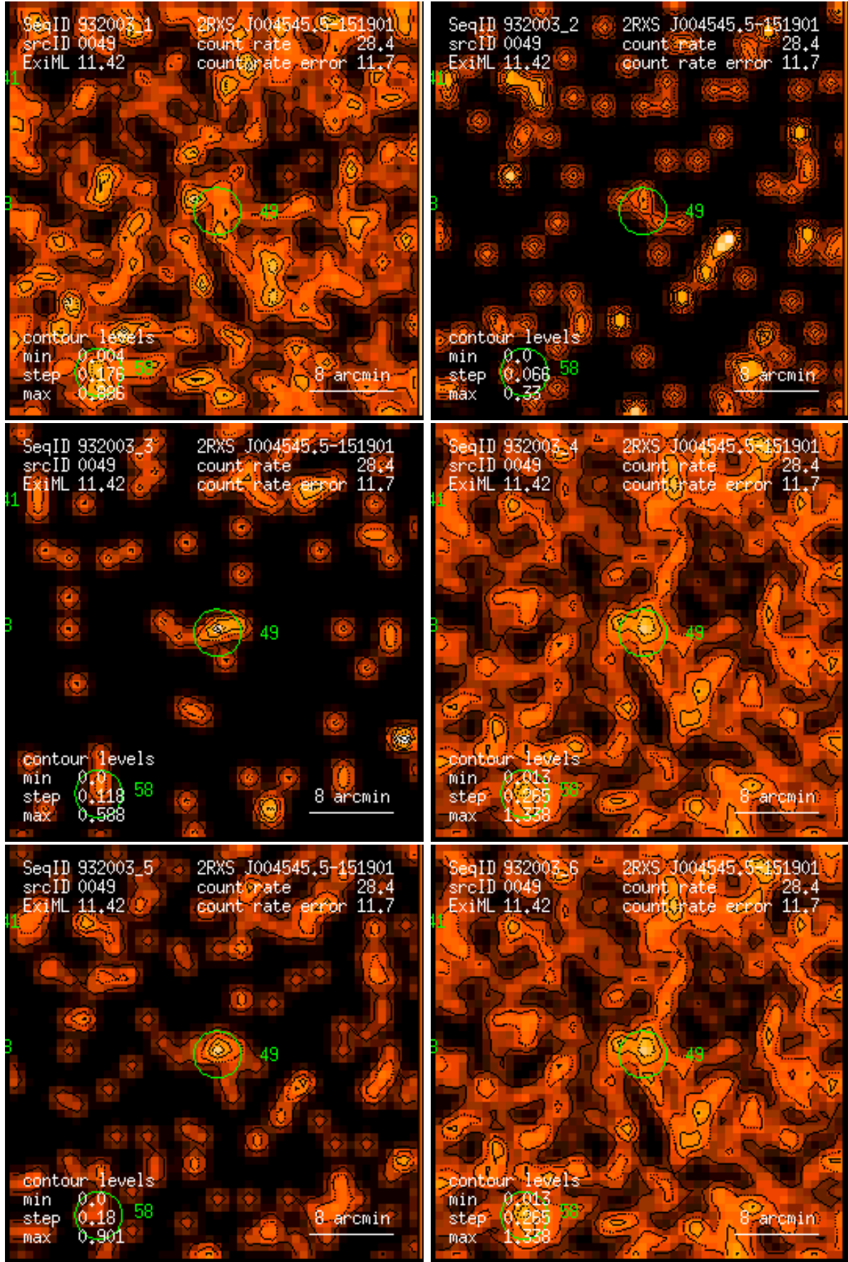
Figure 49: RASS 932003: detection 0049: band rate images, Gaussian filter: (1) PSPC channels 11 – 41, (2) 52 – 90, (3) 91 – 201, (4) 11 – 235, (5) 52 – 201, (6) 11 – 201. Broad band rates in counts/ks. Band rate contour levels in counts/ks/arcmin 2 .
