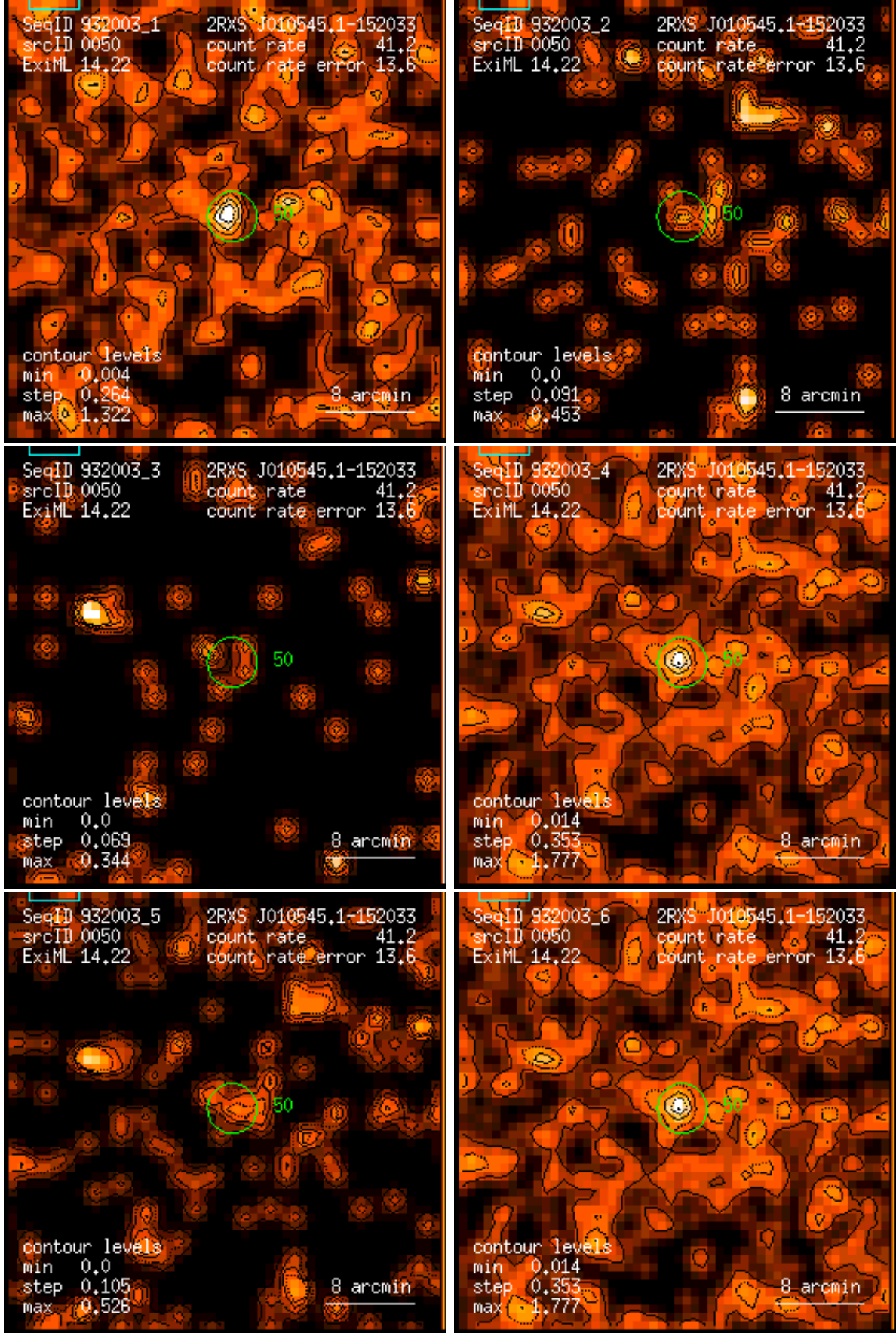
Figure 50: RASS 932003: detection 0050: band rate images, Gaussian filter: (1) PSPC channels 11 – 41, (2) 52 – 90, (3) 91 – 201, (4) 11 – 235, (5) 52 – 201, (6) 11 – 201. Broad band rates in counts/ks. Band rate contour levels in counts/ks/arcmin 2 .
