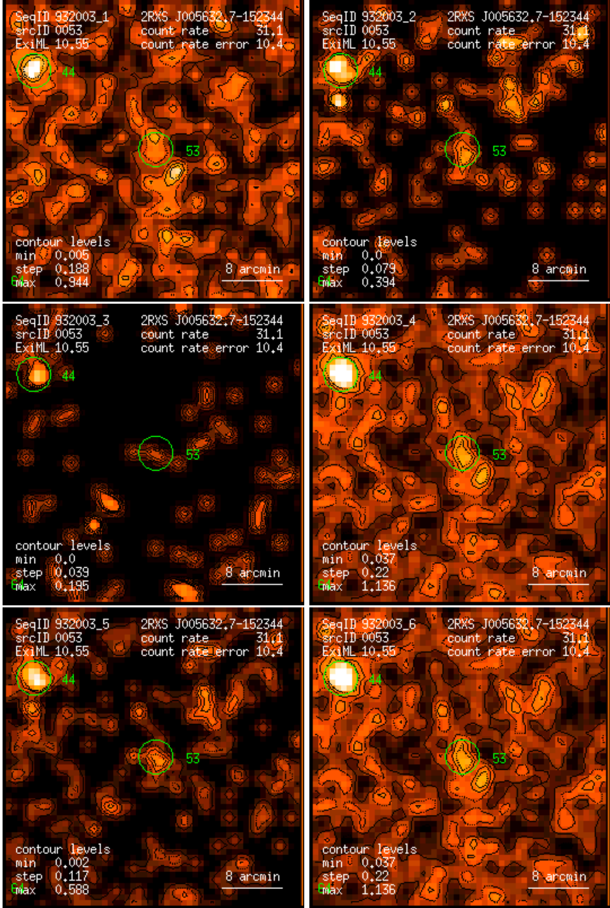
Figure 53: RASS 932003: detection 0053: band rate images, Gaussian filter: (1) PSPC channels 11 – 41, (2) 52 – 90, (3) 91 – 201, (4) 11 – 235, (5) 52 – 201, (6) 11 – 201. Broad band rates in counts/ks. Band rate contour levels in counts/ks/arcmin 2 .
