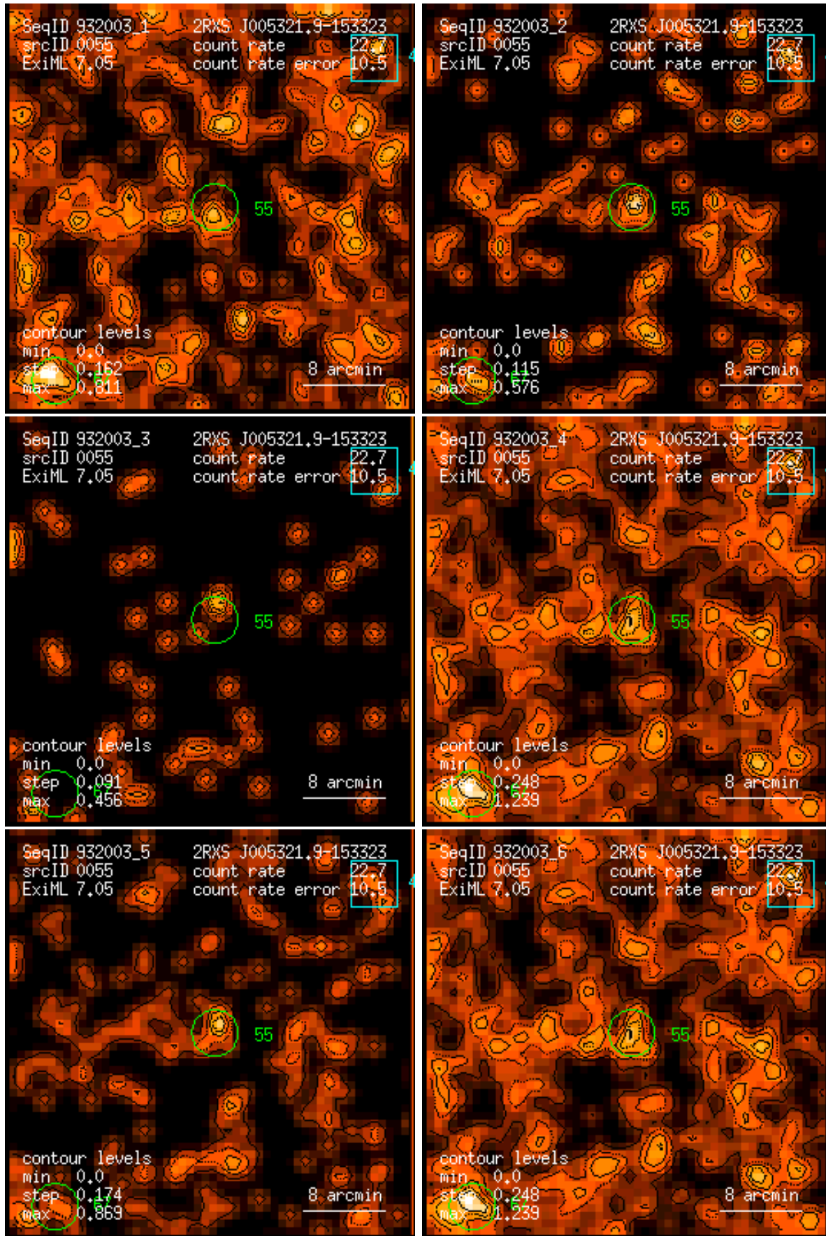
Figure 55: RASS 932003: detection 0055: band rate images, Gaussian filter: (1) PSPC channels 11 – 41, (2) 52 – 90, (3) 91 – 201, (4) 11 – 235, (5) 52 – 201, (6) 11 – 201. Broad band rates in counts/ks. Band rate contour levels in counts/ks/arcmin 2 .
