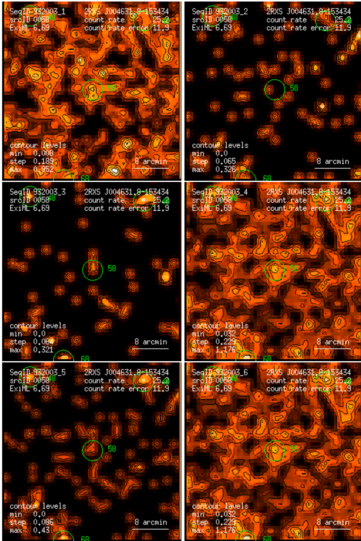
Figure 58: RASS 932003: detection 0058: band rate images, Gaussian filter: (1) PSPC channels 11 – 41, (2) 52 – 90, (3) 91 – 201, (4) 11 – 235, (5) 52 – 201, (6) 11 – 201. Broad band rates in counts/ks. Band rate contour levels in counts/ks/arcmin 2 .
