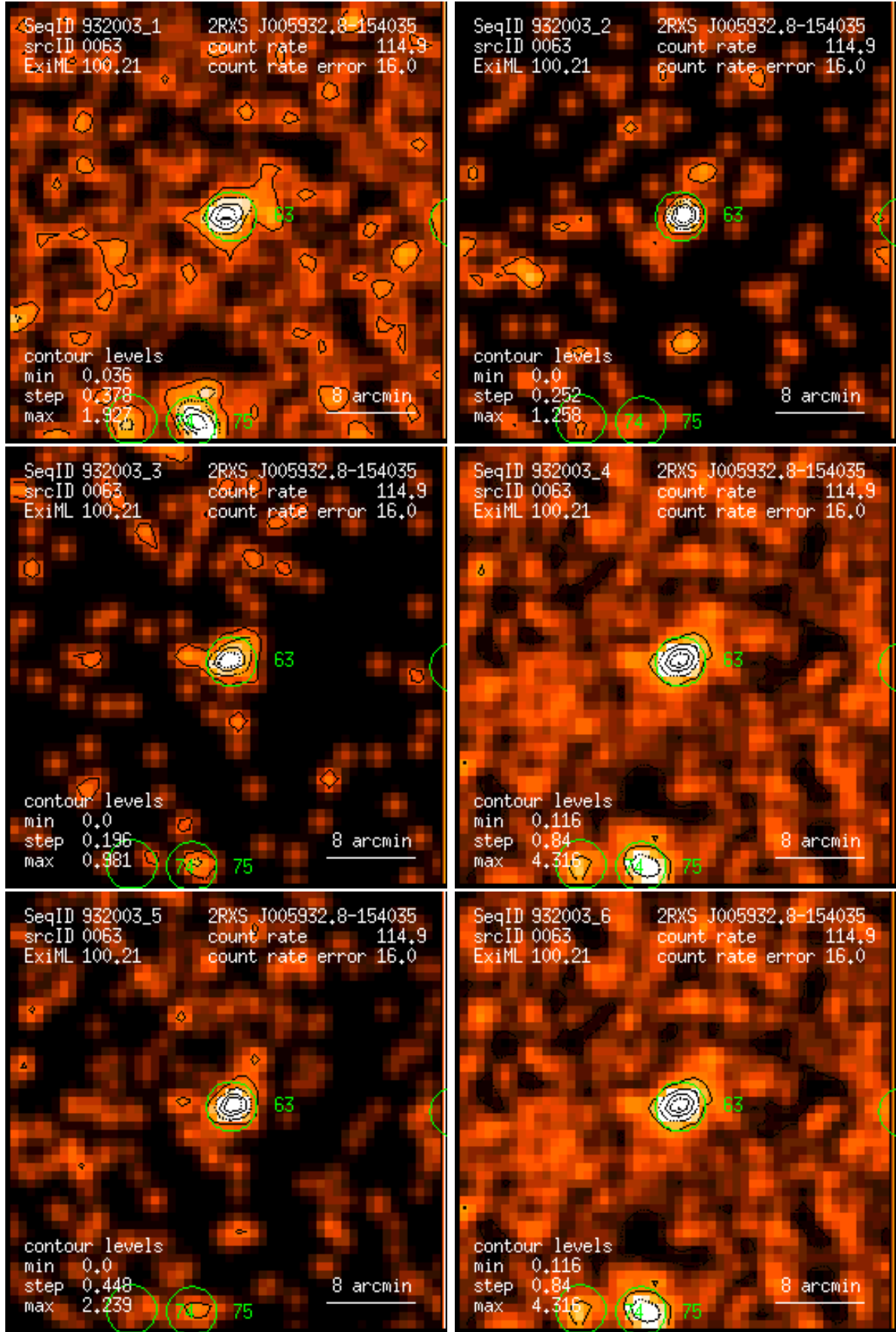
Figure 63: RASS 932003: detection 0063: band rate images, Gaussian filter: (1) PSPC channels 11 – 41, (2) 52 – 90, (3) 91 – 201, (4) 11 – 235, (5) 52 – 201, (6) 11 – 201. Broad band rates in counts/ks. Band rate contour levels in counts/ks/arcmin 2 .
